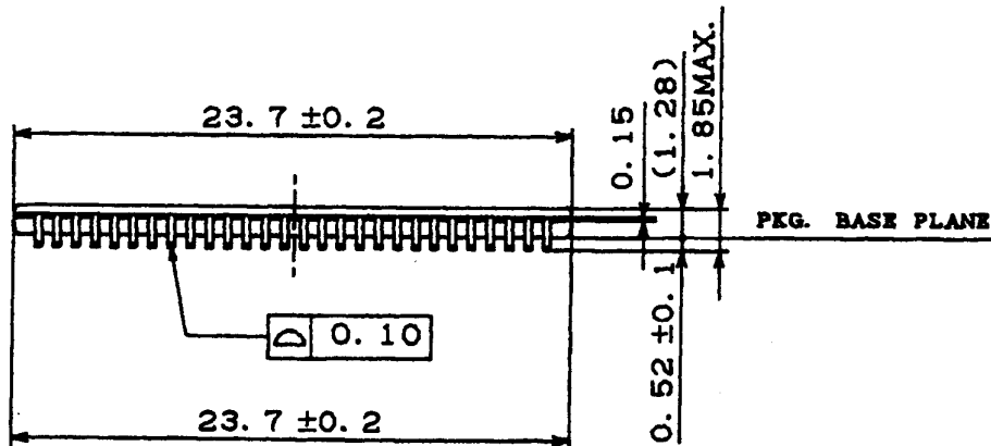
DETAIL A
