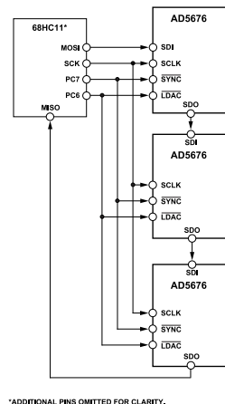
Figure 45. Daisy-Chaining the AD5676
