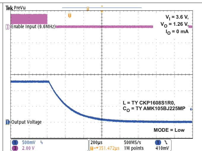
Figure 52. Shut-Down (RF Clock)
