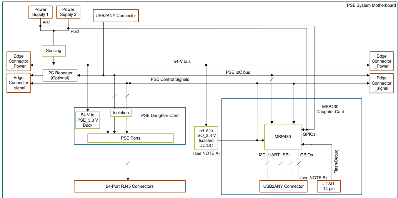
Figure 1. TIDA-050026-23881 Block Diagram
