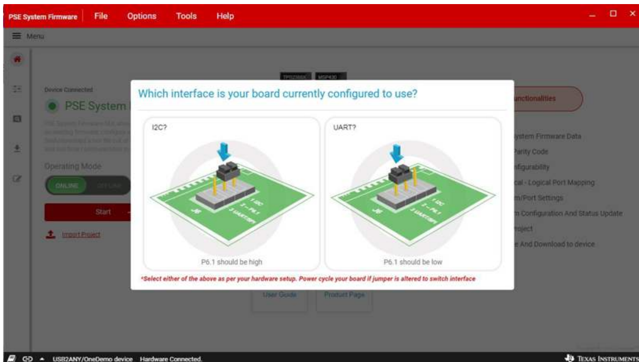
Figure 10. Host Interface Protocol Selection in Online Mode
