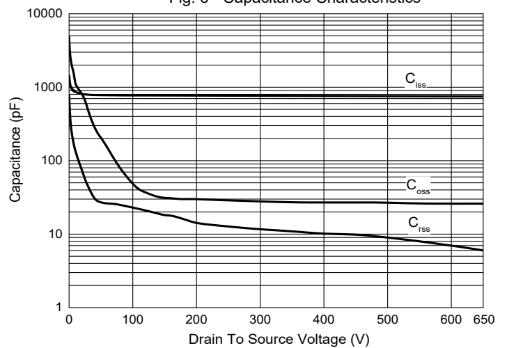
Fig. 6 - Capacitance Characteristics
