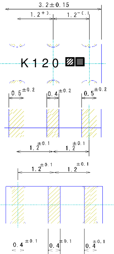
Fig 2 Dimensions Unit: mm
