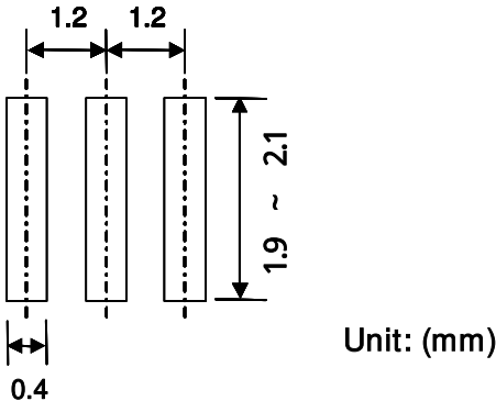
Fig.4 Recommended Land pattern
