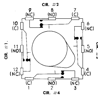
BOTTOM VIEW - SEPARATE MOTOR LEADS NOT SHOWN
