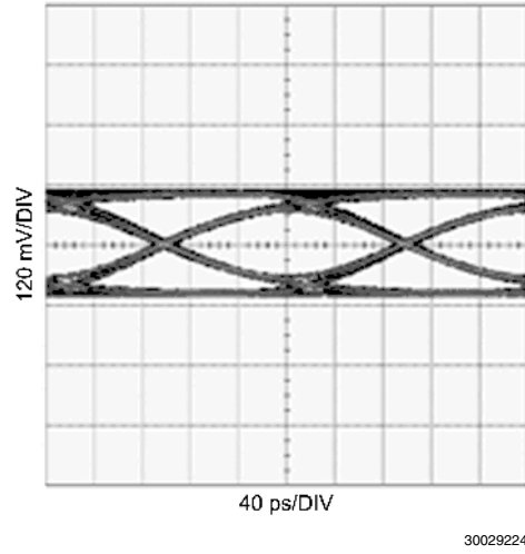
FIGURE 18. Equalized Signal (30in FR4, 5Gbps, PRBS7)
