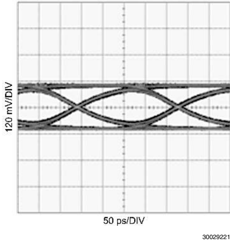
FIGURE 15. Equalized Signal (30in FR4, 4.25Gbps, PRBS7)
