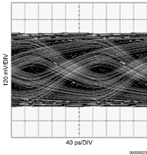
FIGURE 17. Unequalized Signal (30in FR4, 5Gbps, PRBS7)
