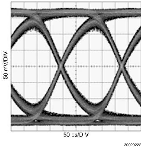
FIGURE 16. Equalized Signal (Zoom) (30in FR4, 4.25Gbps, PRBS7)
