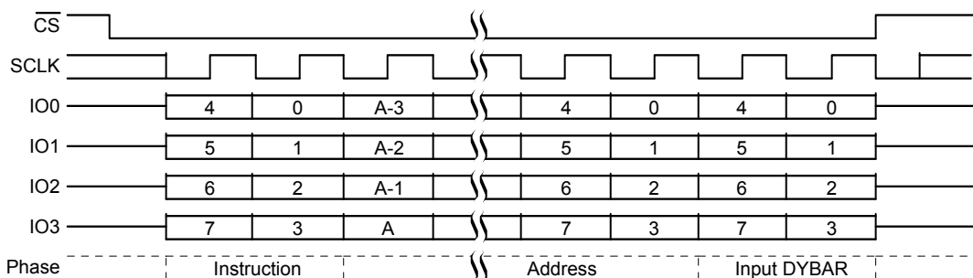
Figure 10.54 DYBWR QPI Mode Command Sequence
