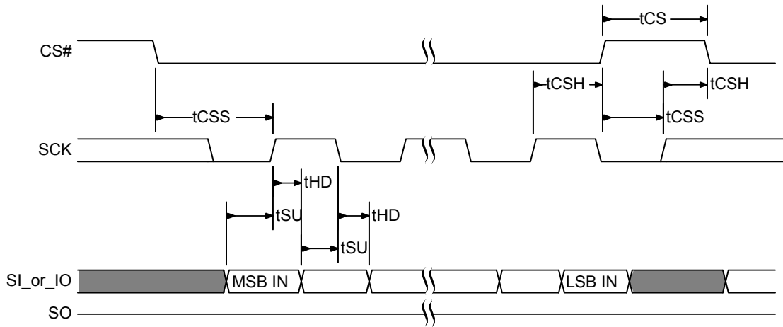
Figure 6.14 SPI DDR Input Timing
