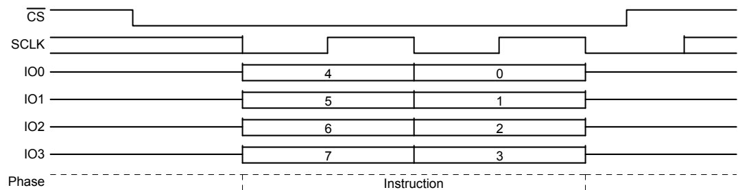
Figure 10.49 Erase or Program Resume Command Sequence QPI Mode
