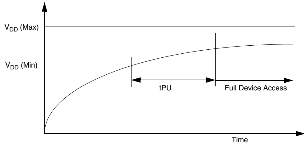
Figure 5.3 Power-up
