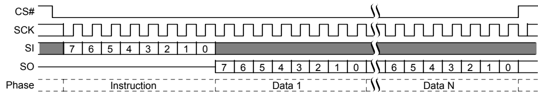
Figure 10.1 Read Identification (RDID) Command Sequence
