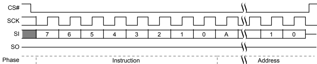
Figure 10.37 Parameter Sector Erase (P4E 20h or 4P4E 21h) Command Sequence
