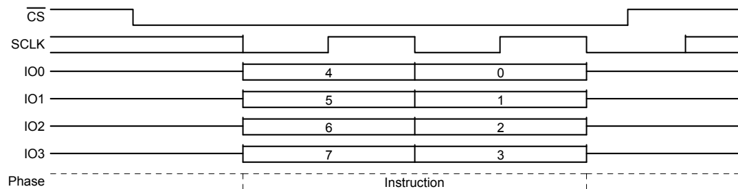
Figure 10.47 Erase or Program Suspend Command Sequence QPI Mode
