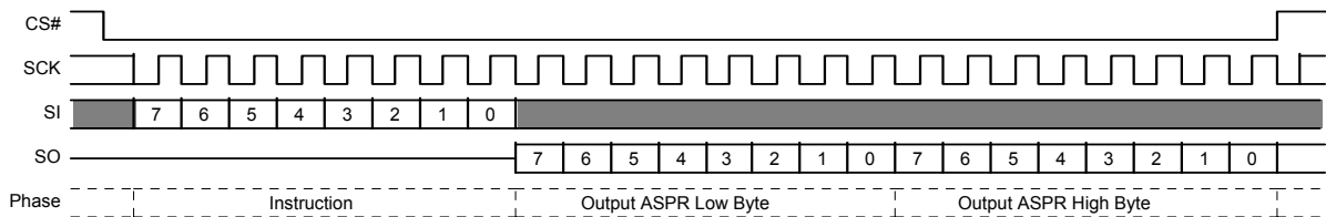
Figure 10.50 ASPRD Command
