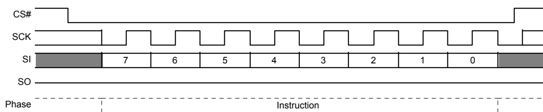
Figure 10.64 Mode Bit Reset Command Sequence
