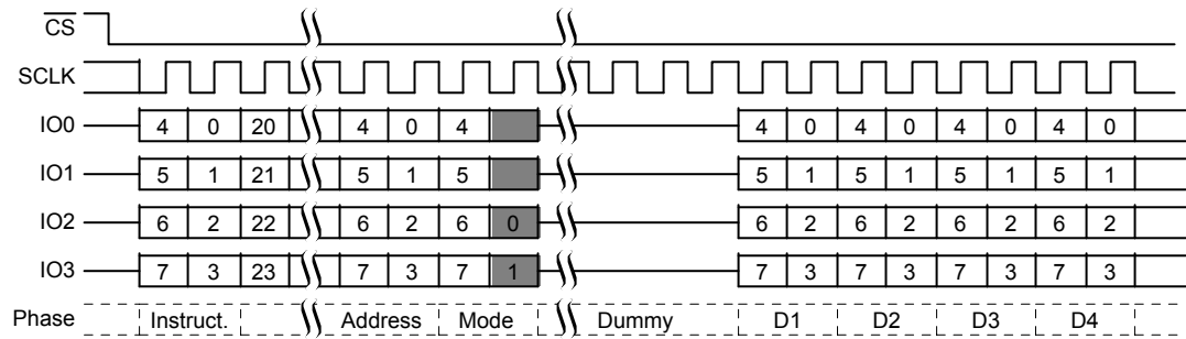
Figure 10.25 Quad I/O Read Command Sequence (3-Byte Address, EBh [CR2V[7]=0]) QPI Mode
