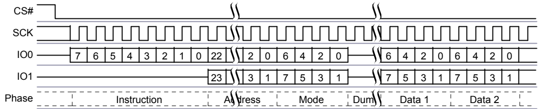
Figure 10.21 Dual I/O Read Command Sequence (3-Byte Address, BBh [CR2V[7]=0])
