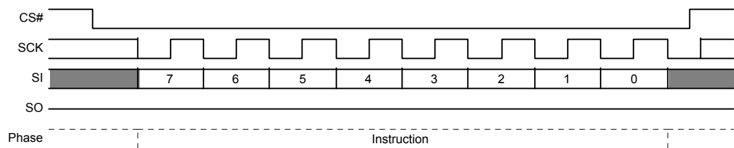
Figure 10.59 PPB Lock Bit Write Command Sequence
