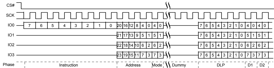
Figure 10.31 Continuous DDR Quad I/O Read Subsequent Access (3-Byte Address)
