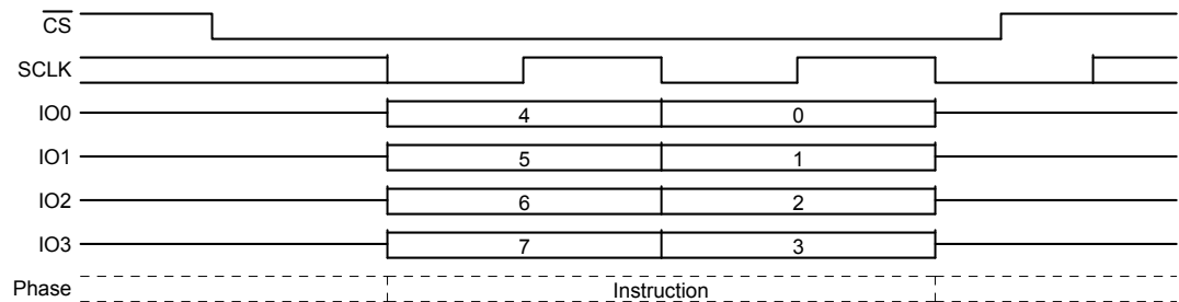
Figure 10.11 Clear Status Register (CLSR) Command Sequence QPI Mode
