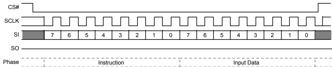
Figure 10.18 Set Burst Length Command Sequence
