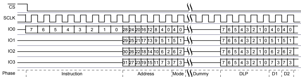
Figure 4.11 DDR Quad I/O Read
