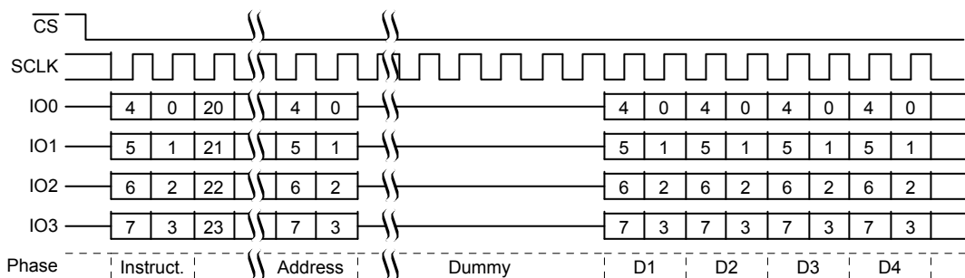
Figure 10.5 RSFDP QPI Mode Command Sequence
