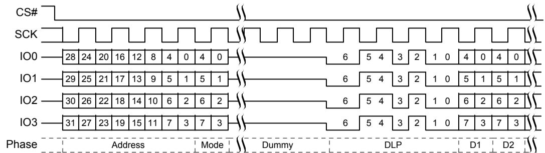
Figure 10.34 Continuous DDR Quad I/O Read Subsequent Access (4-Byte Address)
