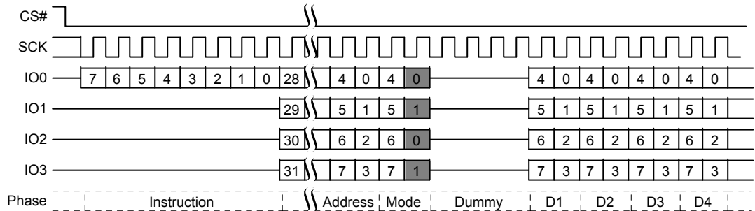
Figure 10.27 Quad I/O Read Command Sequence (4-Byte Address, ECh or EBh [CR2V[7]=1])
