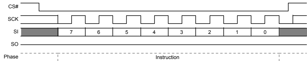
Figure 10.48 Erase or Program Resume Command Sequence
