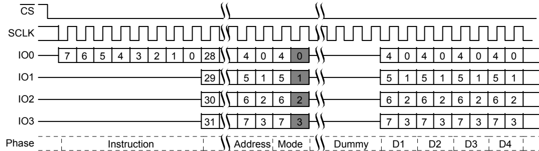
Figure 4.9 Quad I/O Command
