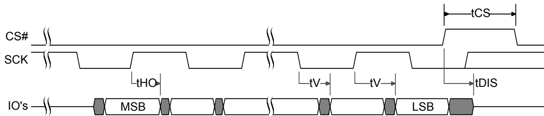
Figure 6.15 SPI DDR Output Timing
