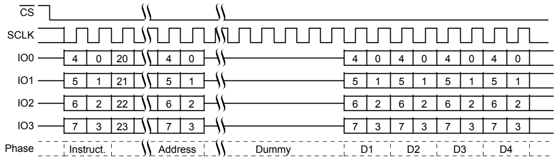
Figure 10.16 Read Any Register, QPI Mode, CR2[7] = 0, Command Sequence
