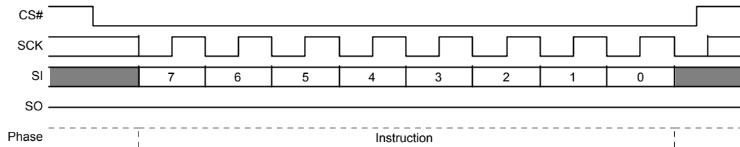
Figure 10.14 Enter 4 Byte Address Mode (4BAM B7h) Command Sequence
