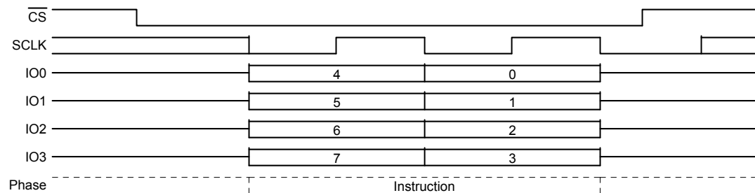
Figure 10.67 DPD Command Sequence QPI Mode
