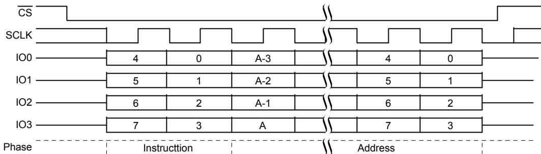
Figure 10.38 Parameter Sector Erase (P4E 20h or 4P4E 21h) QPI Mode Command Sequence
