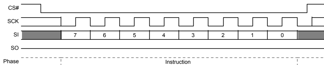
Figure 10.6 Write Enable (WREN) Command Sequence
