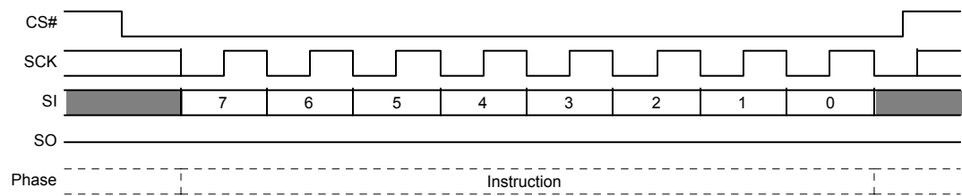
Figure 10.10 Clear Status Register (CLSR) Command Sequence
