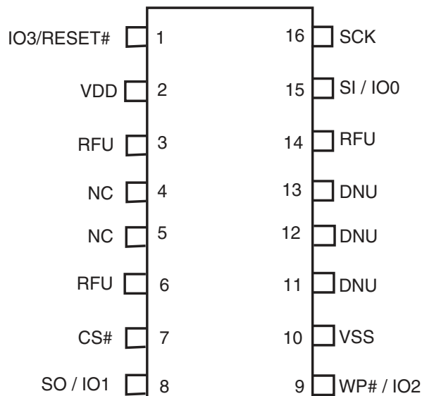
Figure 7.1 16-Lead SOIC Package, Top View
