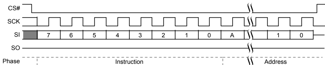
Figure 10.39 Sector Erase (SE D8h or 4SE DCh) Command Sequence
