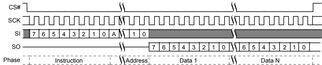
Figure 10.19 Read Command Sequence (3-Byte Address, 03h or 13h)
