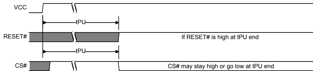
Figure 6.6 POR followed by Hardware Reset
