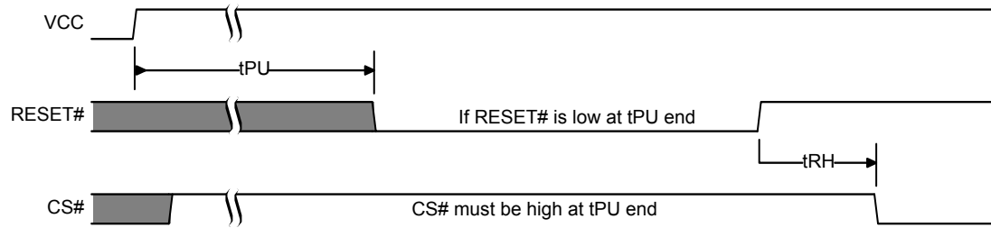
Figure 6.5 Reset high at the end of POR
