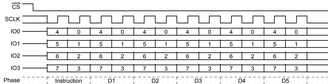
Figure 10.2 Read Identification (RDID) QPI Mode Command
