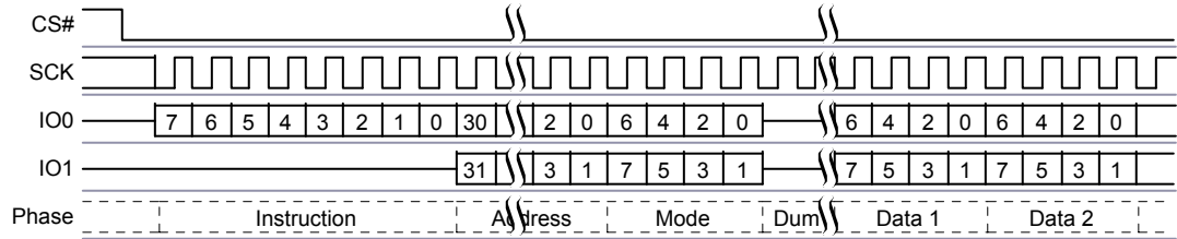
Figure 10.22 Dual I/O Read Command Sequence (4-Byte Address, BBh [CR2V[7]=1])
