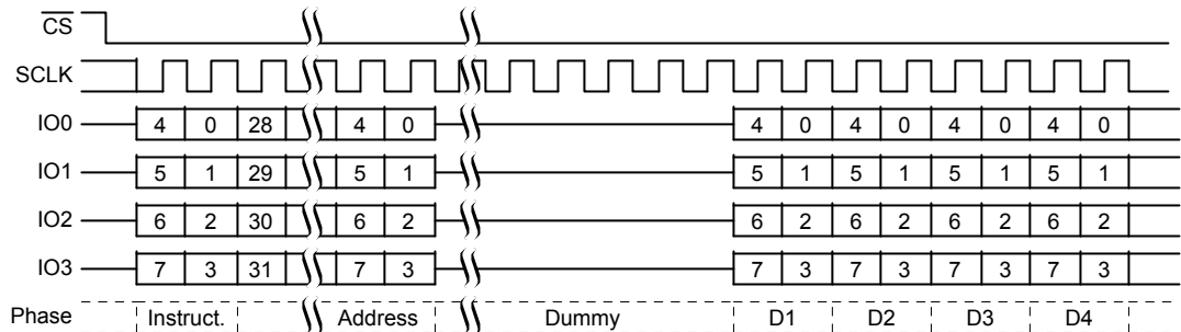
Figure 10.17 Read Any Register, QPI Mode, CR2[7] = 1 Command Sequence
