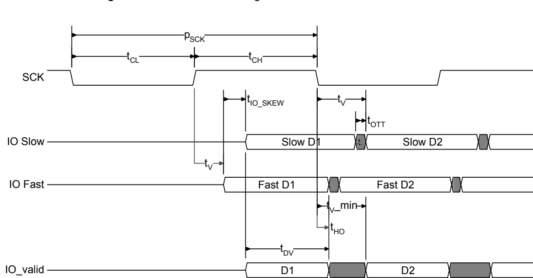
Figure 6.16 SPI Data Learning Pattern DDR Data Valid Window
