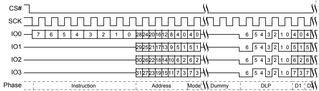
Figure 10.32 DDR Quad I/O Read Initial Access (4-Byte Address, EEh or EDh [CR2V[7]=1])
