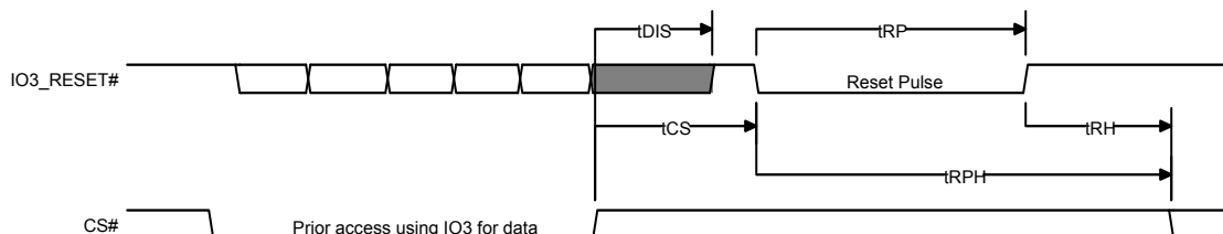
Figure 6.8 Hardware Reset when Quad Mode and IO3 / Reset# are Enabled
