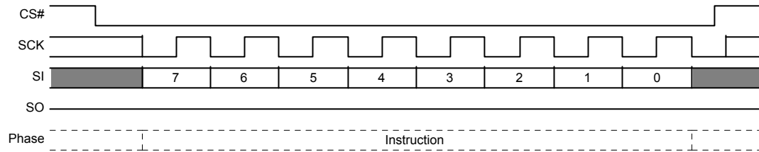
Figure 10.8 Write Disable (WRDI) Command Sequence
