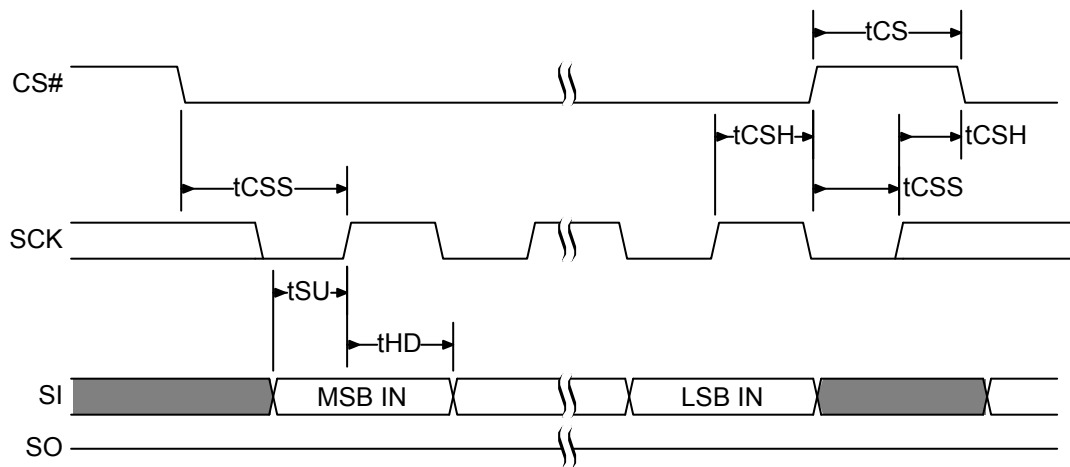
Figure 6.10 SPI Single Bit Input Timing
