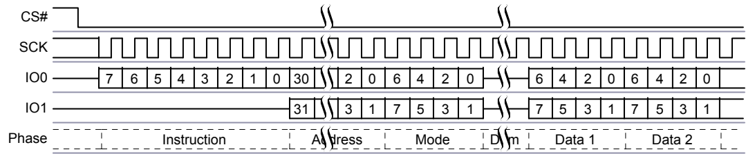
Figure 4.8 Dual I/O Command
