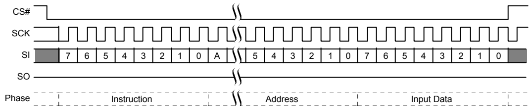
Figure 10.53 DYBWR Command Sequence
