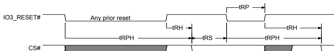
Figure 6.7 Hardware Reset when Quad Mode is not enabled and IO3 / Reset# is Enabled
