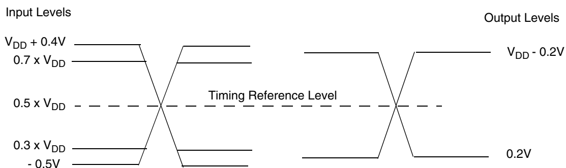
Figure 6.3 Input, Output, and Timing Reference Levels
