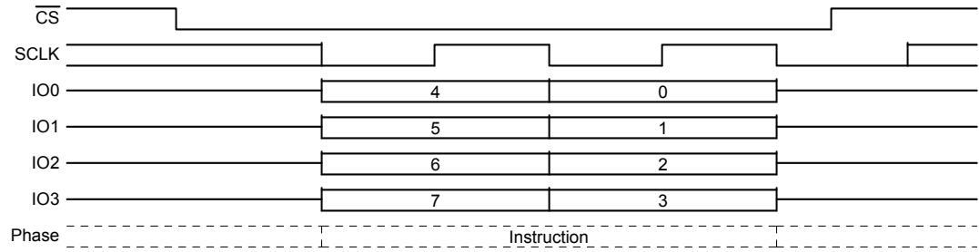
Figure 10.7 Write Enable (WREN) Command Sequence QPI Mode
