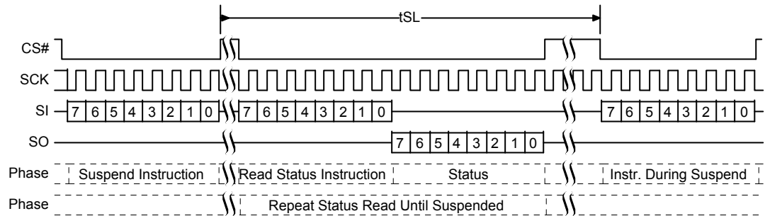
Figure 10.45 Program or Erase Suspend Command Sequence
