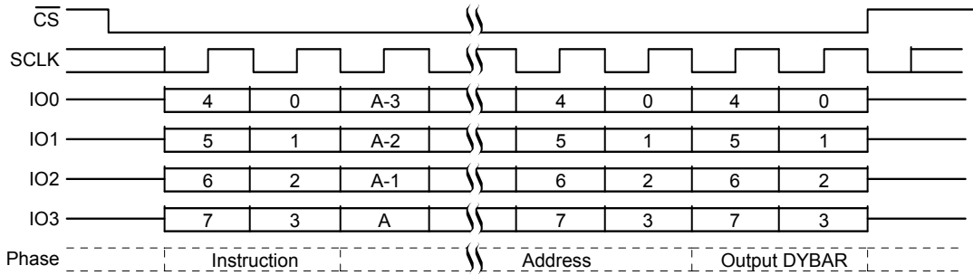
Figure 10.52 DYBRD QPI Mode Command Sequence
