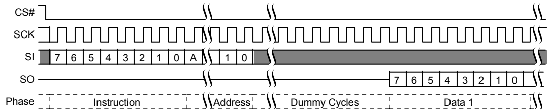
Figure 10.15 Read Any Register Read Command Sequence
