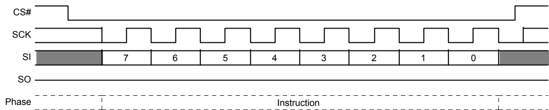
Figure 10.57 PPB Erase Command Sequence
