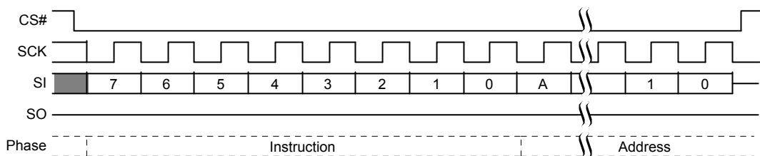
Figure 10.43 EES Command Sequence
