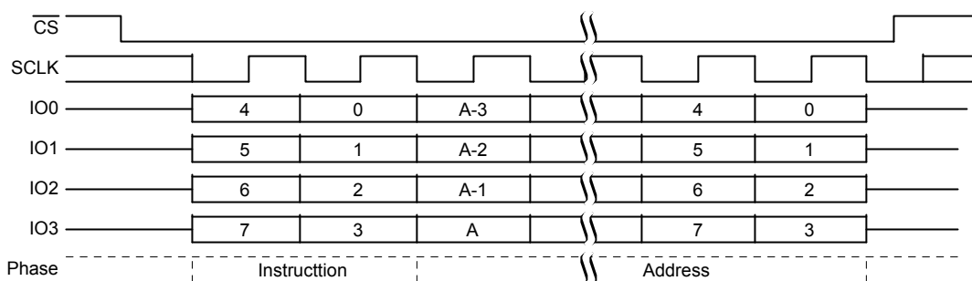
Figure 10.44 EES QPI Mode Command Sequence
