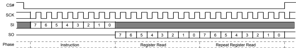
Figure 10.58 PPB Lock Register Read Command Sequence
