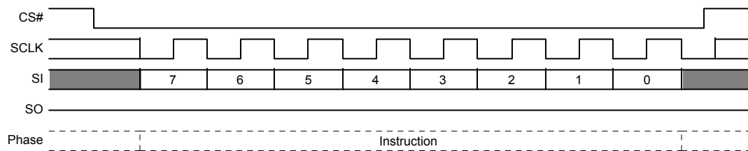
Figure 10.66 Deep Power-down Command Sequence
