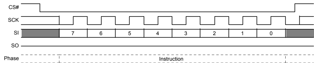
Figure 10.62 Software Reset Command Sequence
