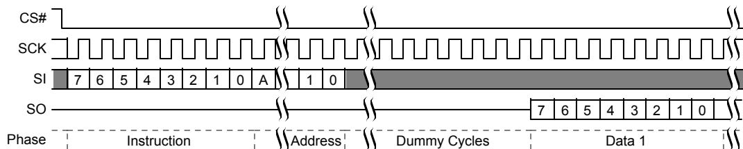
Figure 10.20 Fast Read (FAST_READ) Command Sequence (3-Byte Address, 0Bh [CR2V[7]=0])
