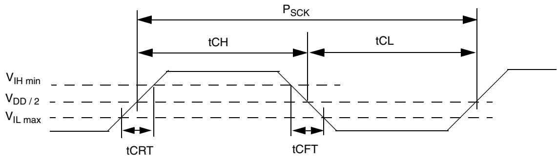
Figure 6.9 Clock Timing
