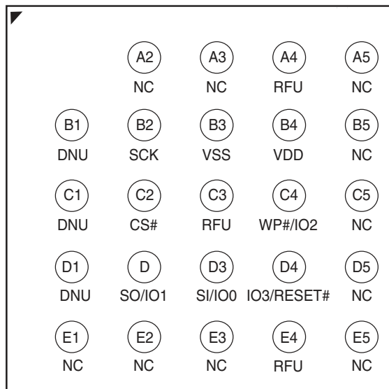
Figure 7.2 24-Ball BGA, 5x5 Ball Footprint (FAB024), Top View
