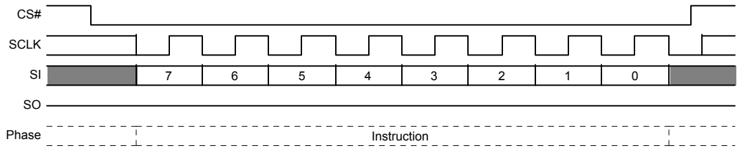
Figure 10.68 Release from Deep Power-down Command Sequence
