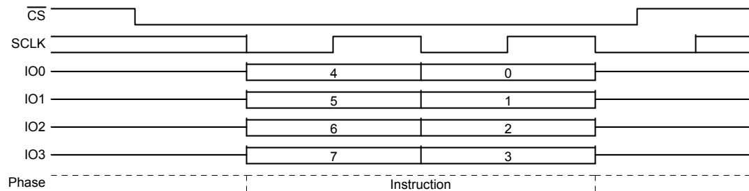
Figure 10.63 Software Reset Command Sequence QPI Mode
