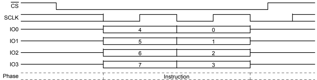
Figure 10.69 RES Command Sequence QPI Mode
