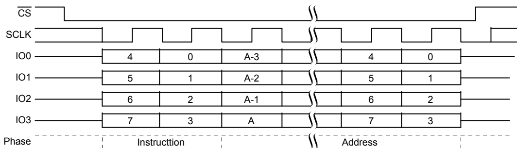
Figure 10.40 Sector Erase (SE D8h or 4SE DCh) QPI Mode Command Sequence
