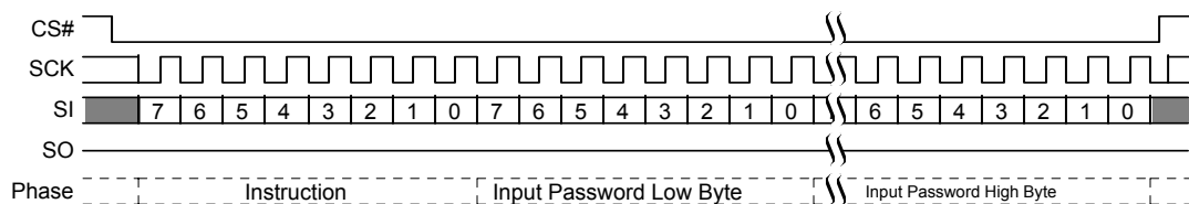
Figure 10.61 Password Unlock Command Sequence
