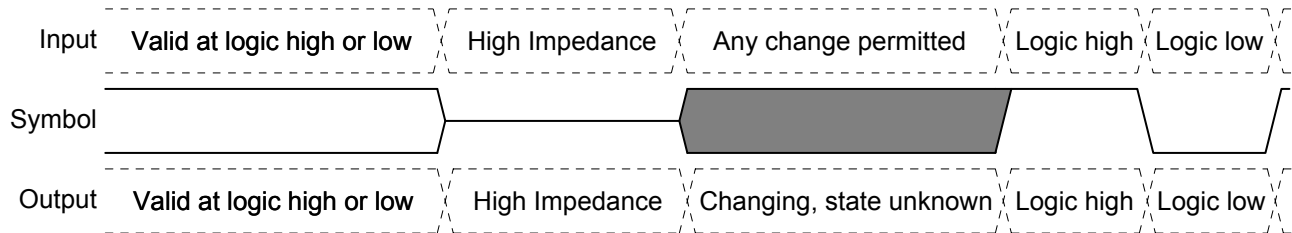
Figure 6.1 Waveform Element Meanings
