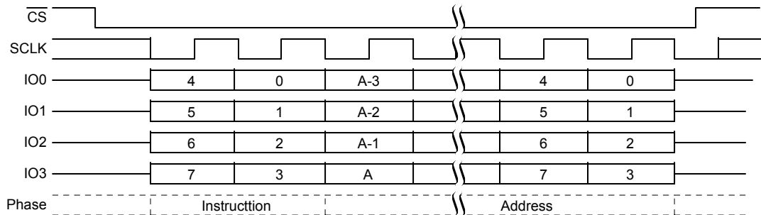
Figure 10.42 Bulk Erase Addressed Command Sequence QPI Mode
