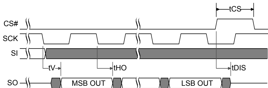
Figure 6.11 SPI Single Bit Output Timing
