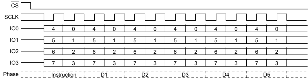
Figure 10.3 Read Quad Identification (RDQID) Command Sequence
