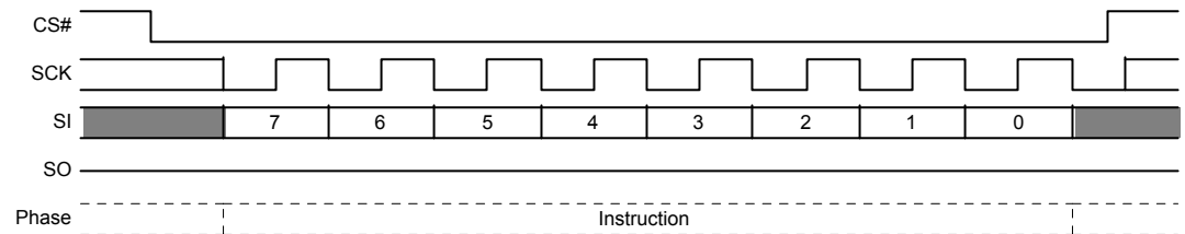
Figure 10.46 Erase or Program Suspend Command Sequence
