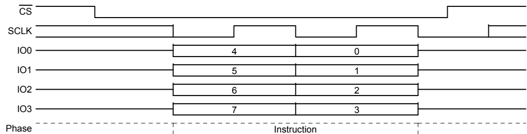
Figure 10.9 Write Disable (WRDI) Command Sequence QPI Mode
