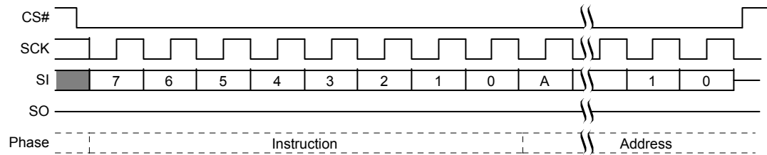
Figure 10.56 PPBP Command Sequence
