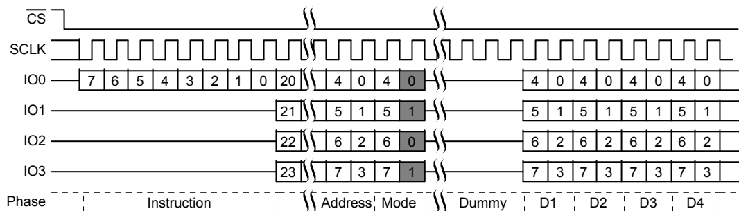
Figure 10.24 Quad I/O Read Command Sequence (3-Byte Address, EBh [CR2V[7]=0])
