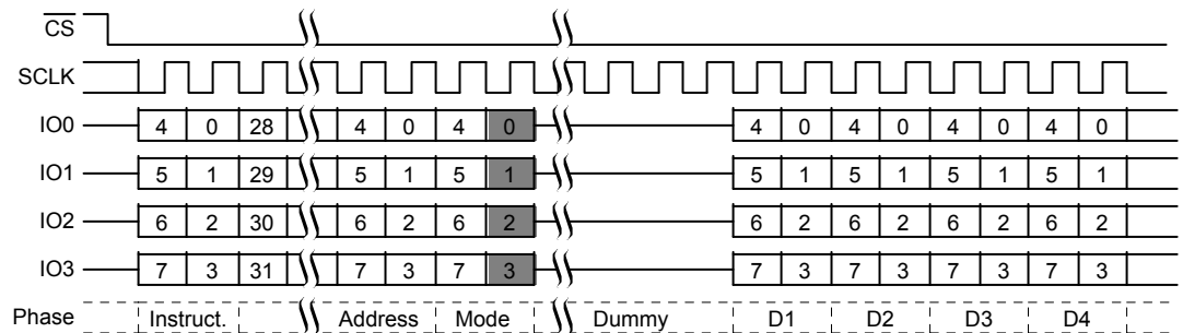
Figure 4.10 Quad I/O Read Command in QPI Mode
