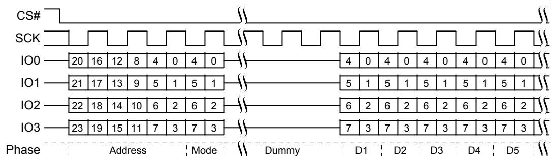
Figure 10.31 Continuous DDR Quad I/O Read Subsequent Access (3-Byte Address)
