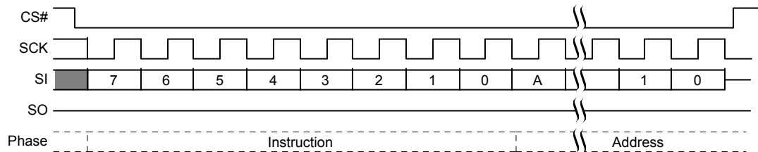
Figure 10.41 Bulk Erase Addressed Command Sequence
