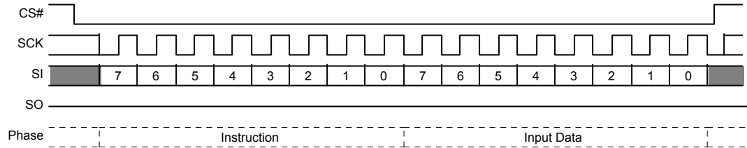
Figure 10.12 Write VDLR (WVDLR) Command Sequence
