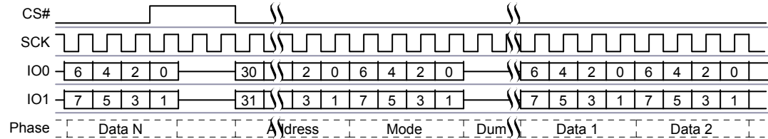
Figure 10.23 Dual I/O Continuous Read Command Sequence (4-Byte Address [CR2V[7]=1])
