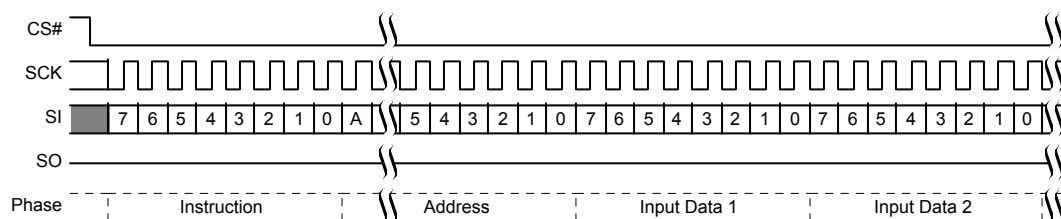
Figure 10.35 Page Program (PP 02h or 4PP 12h) Command Sequence
