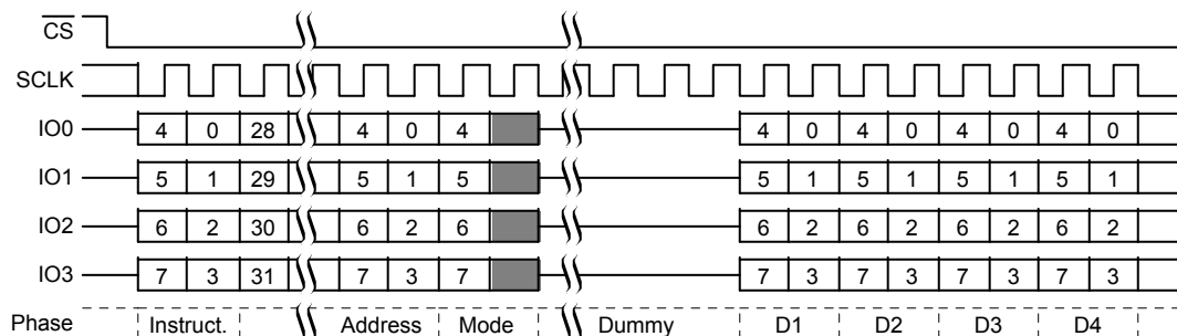
Figure 10.29 Quad I/O Read Command Seq. (4-Byte Address, ECh or EBh [CR2V[7]=1]) QPI Mode
