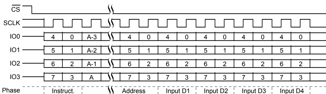
Figure 10.36 Page Program (PP 02h or 4PP 12h) QPI Mode Command Sequence
