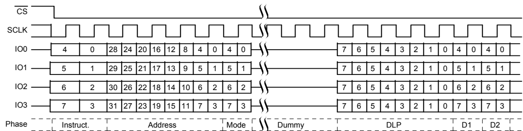
Figure 10.33 DDR Quad I/O Read Initial Access (4-Byte Address, EEh or EDh [CR2V[7]=1]) QPI Mode
