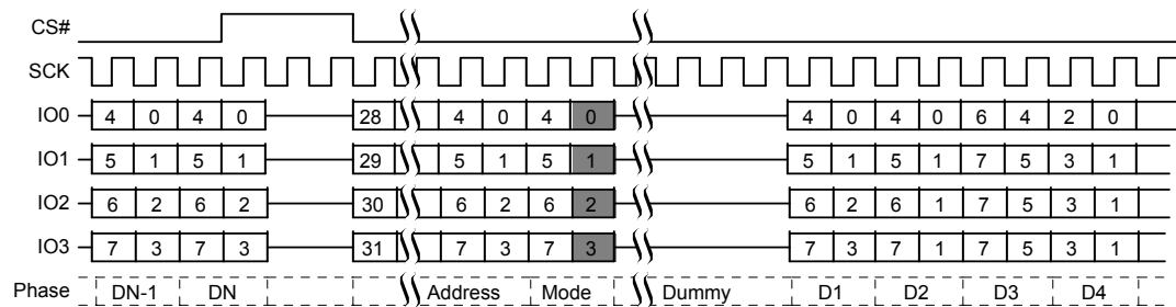
Figure 10.28 Continuous Quad I/O Read Command Sequence (4-Byte Address)
