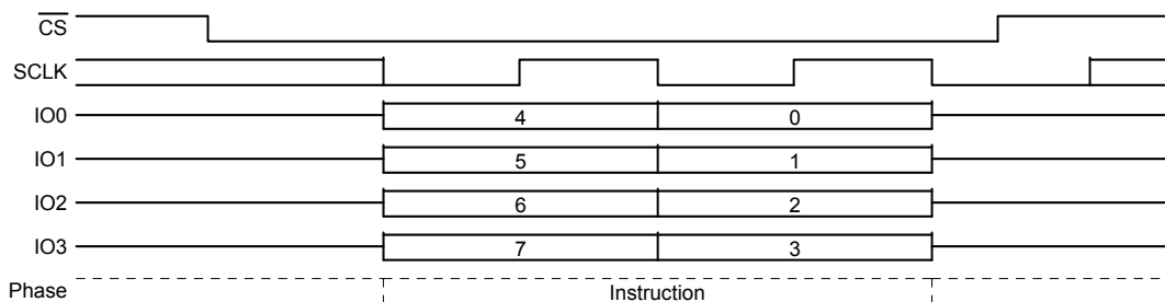
Figure 10.65 Mode Bit Reset Command Sequence QPI Mode
