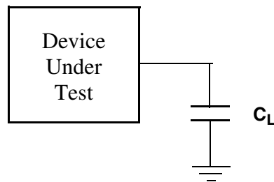
Figure 6.2 Test Setup
