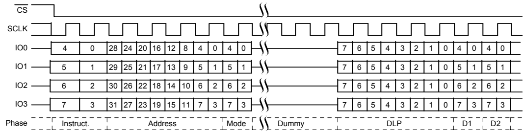
Figure 4.12 DDR Quad I/O Read in QPI Mode
