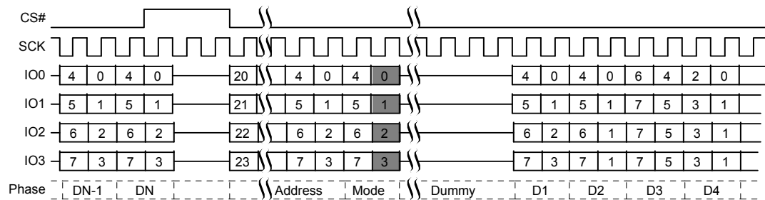
Figure 10.26 Continuous Quad I/O Read Command Sequence (3-Byte Address)
