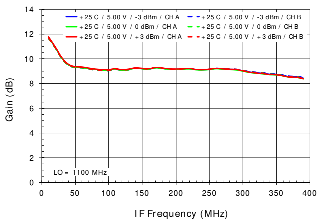
IF Gain flatness vs. LO Power [ G_{MIXR\_T} , HS injection]
