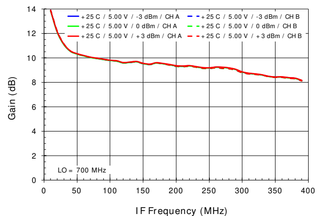
IF Gain flatness vs. LO Power [ G_{MIXR\_T} , LS injection]
