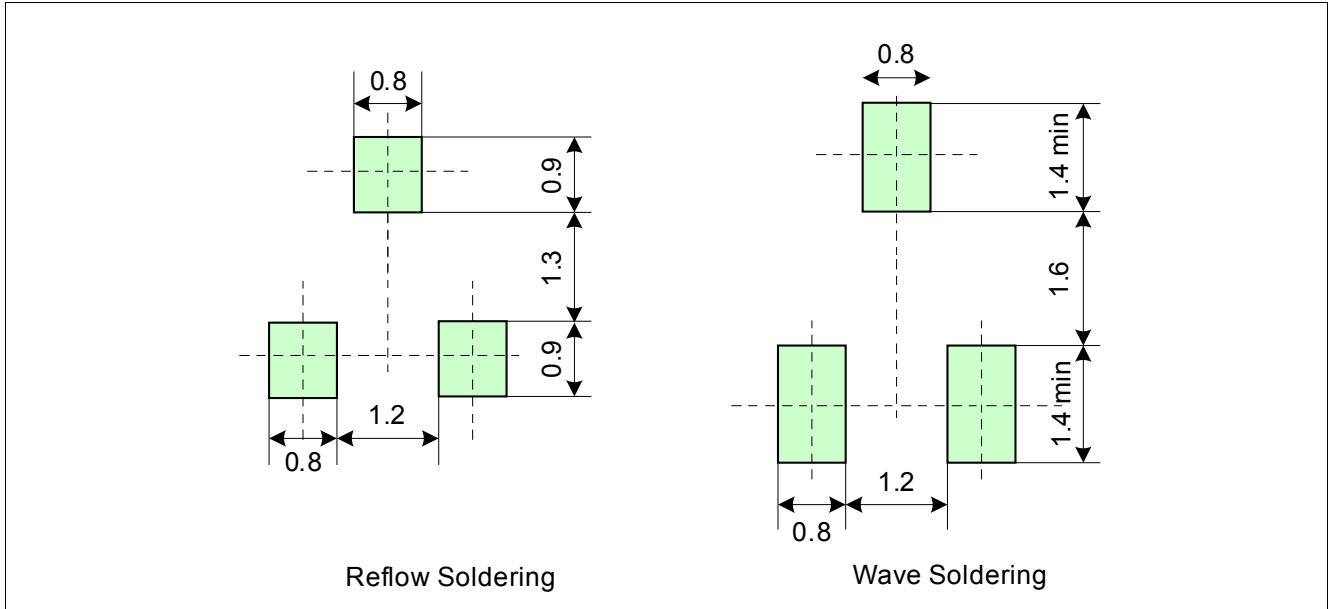
Figure 8 Footprint PG-SC59-3-5
