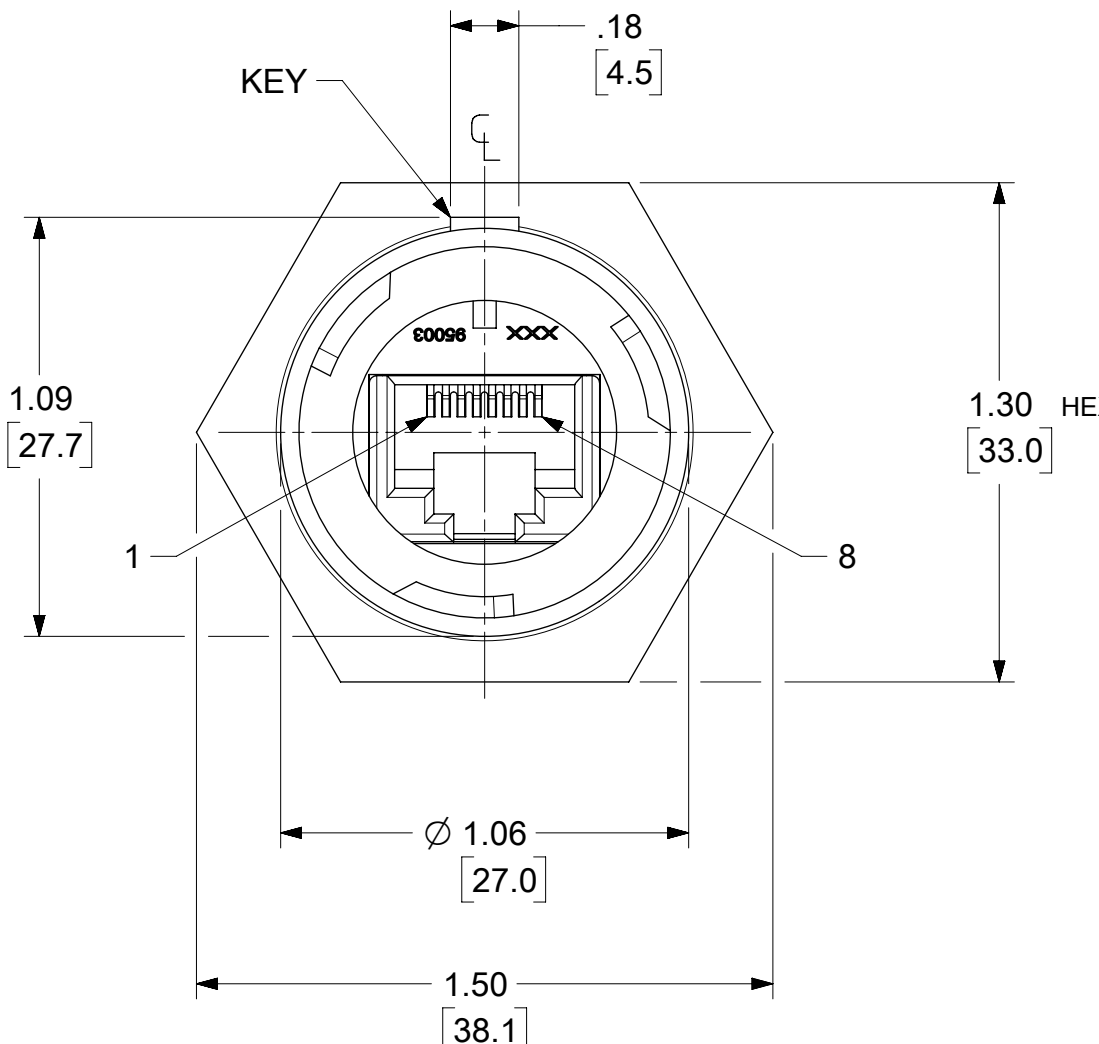
RJ45 FACE VIEW REF. TIA/EIA 568B
