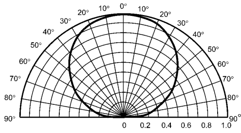
Fig. 8.7 Radiation Pattern
