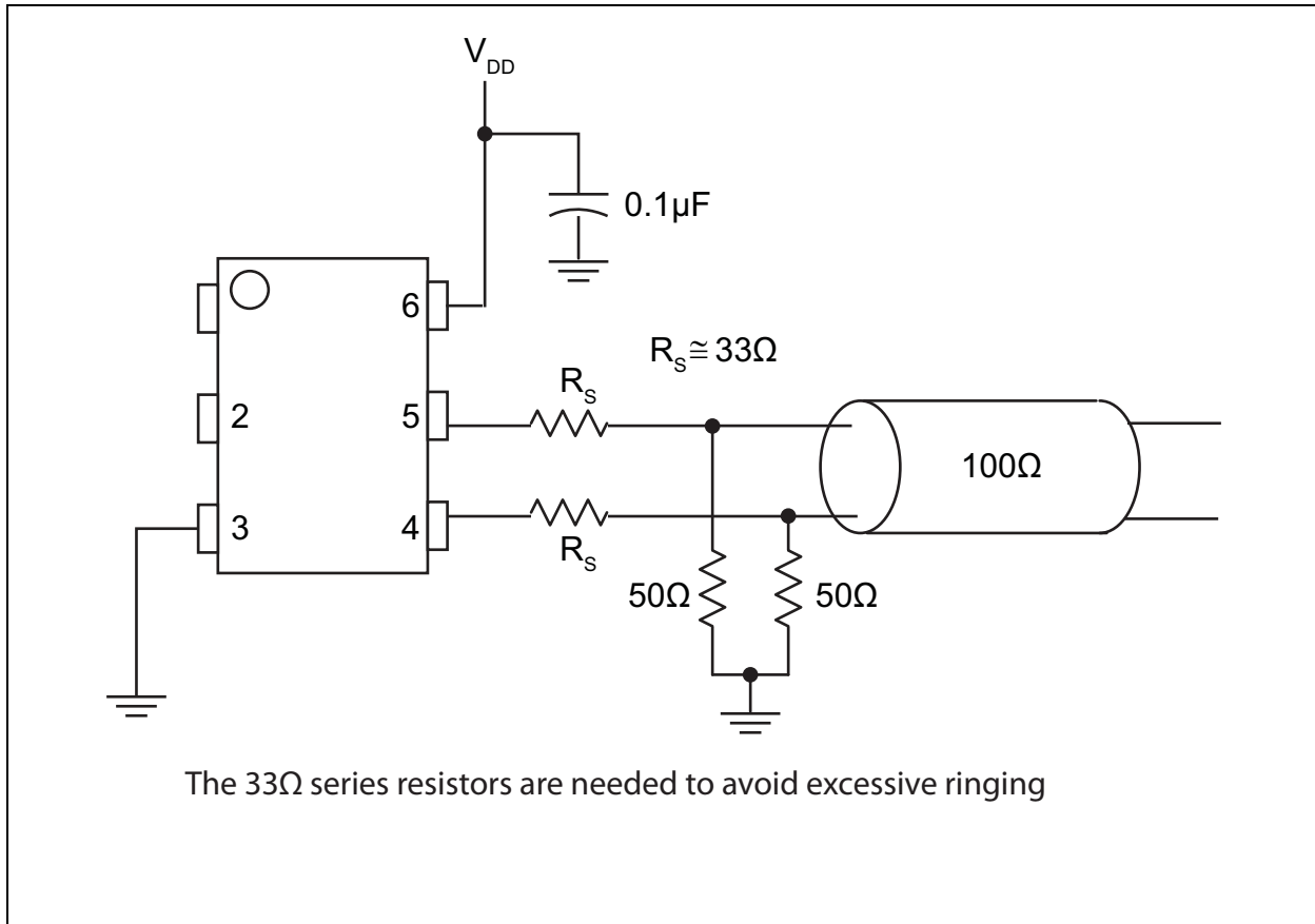
FIGURE 3-3: HCSSL Termination (DSA12x4).
