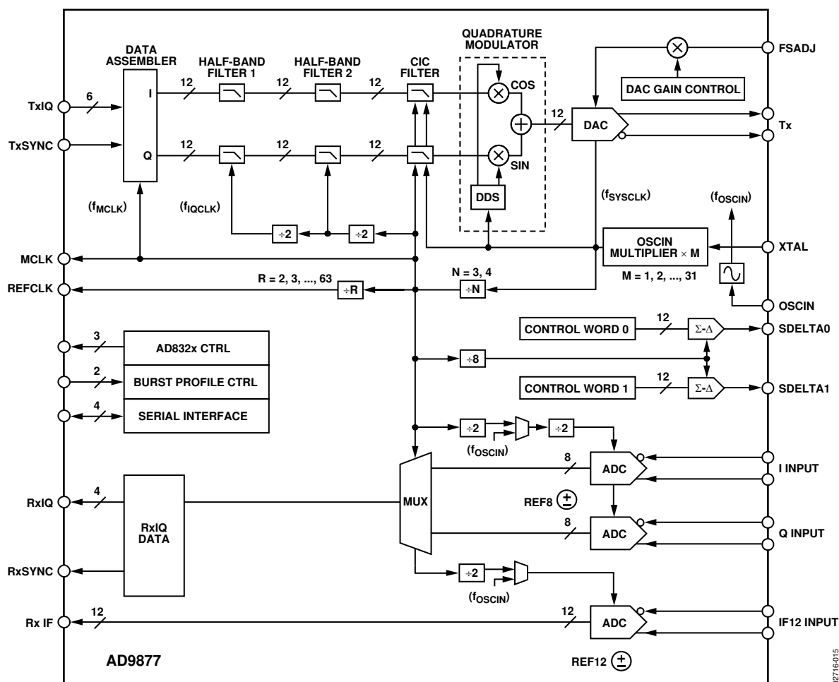
Figure 15. Block Diagram
