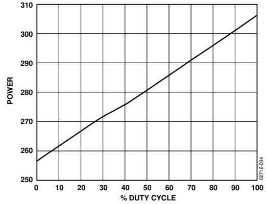
Figure 4. Power Consumption vs. Transmit Burst Duty Cycle
