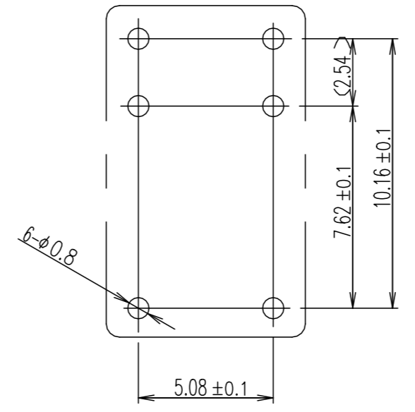
DRILLING DIAGRAM (BOTTOM VIEW)
