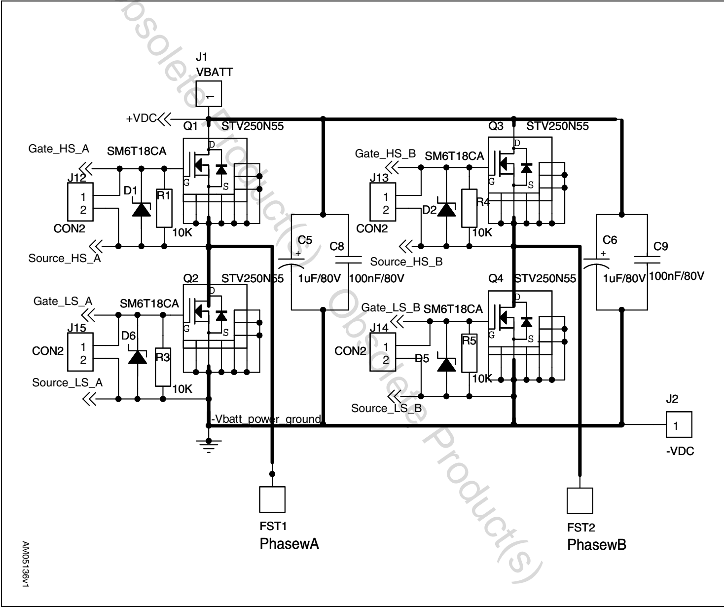
Figure 3. Power board
