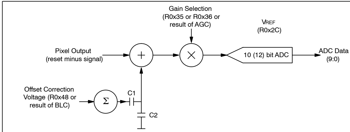
Figure 20. Signal Path
