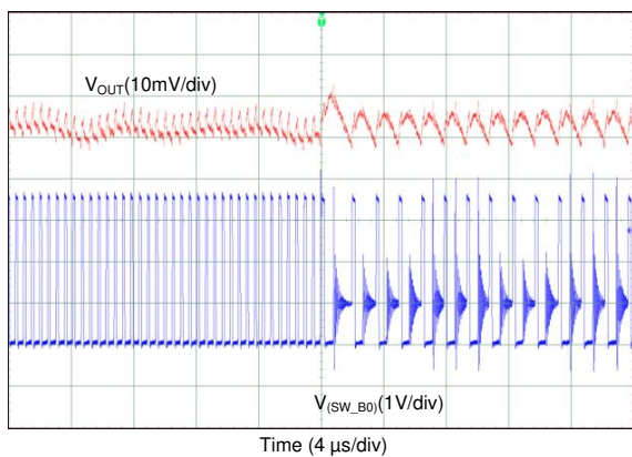
Figure 92. Transient from PWM-to-PFM Mode (1-Phase Output)
