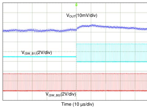
Figure 93. Transient from 1-Phase to 2-Phase Operation (4-Phase Output)
