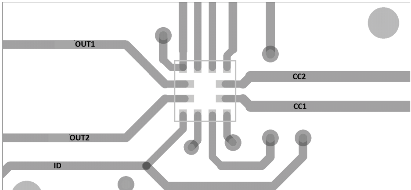
Figure 6. TUSB321 Layout
