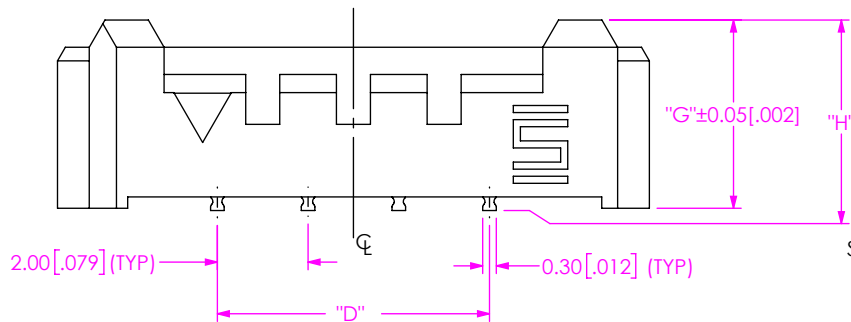
FIG 1 UMPS-04-03.5-XX-V-S SHOWN
