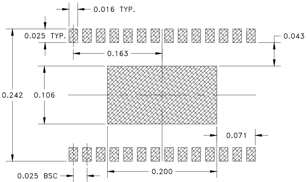
Figure 19: Solder Mask Outline
