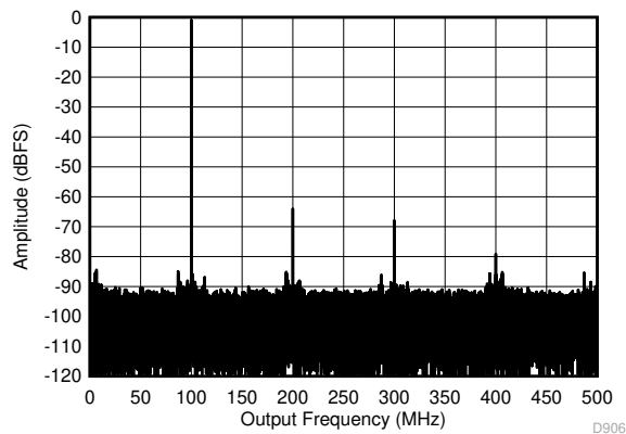
F_S = 1000\text{MSPS} , Low Power Mode Figure 7-11. Single Tone FFT at 99.997 MHz and -1 dBFS
