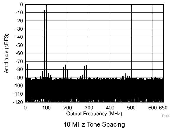
Figure 7-48. Two Tone FFT at 95.07 MHz Center
