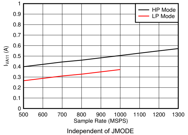
Figure 7-86. Quad Channel, I_{VA11} vs FS
