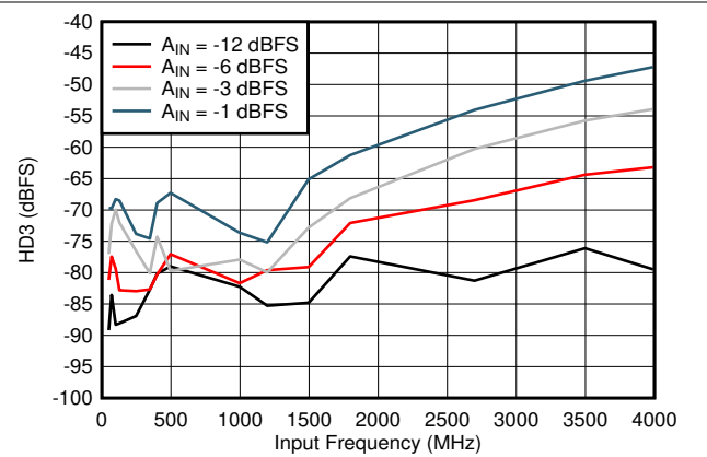
Figure 7-20. HD3 vs Input Frequency
