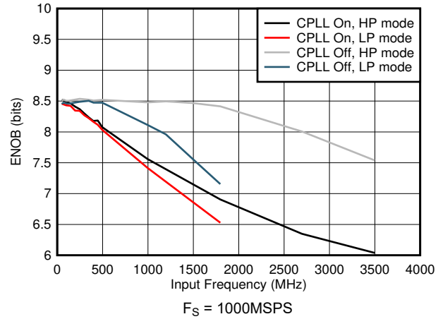
Figure 7-68. ENOB vs Input Frequency and CPLL
