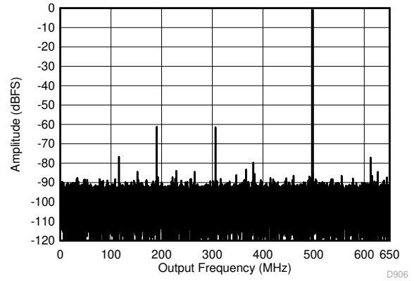
Figure 7-8. Single Tone FFT at 1797 MHz and -1 dBFS
