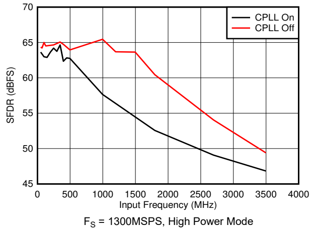
Figure 7-62. SFDR vs Input Frequency and CPLL
