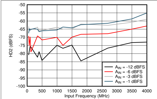
Figure 7-19. HD2 vs Input Frequency
