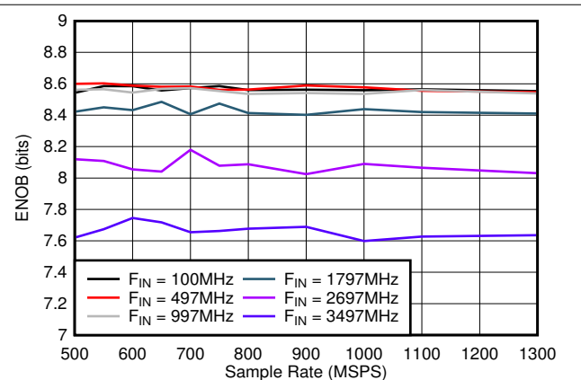
Figure 7-24. ENOB vs Sample Rate
