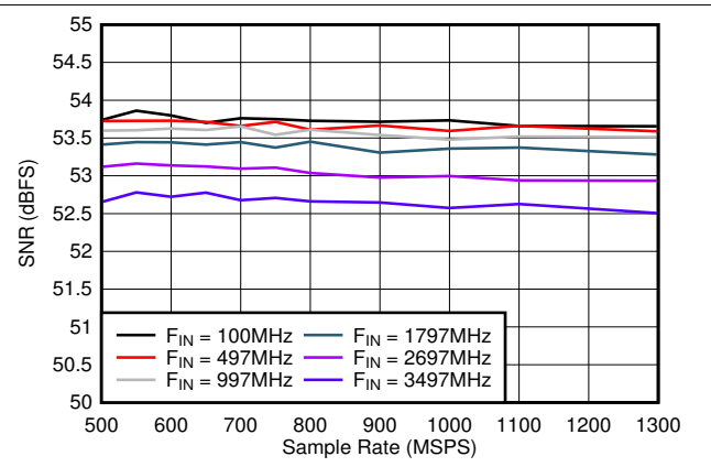
Figure 7-22. SNR vs Sample Rate
