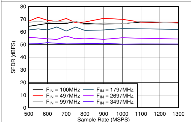
Figure 7-21. SFDR vs Sample Rate
