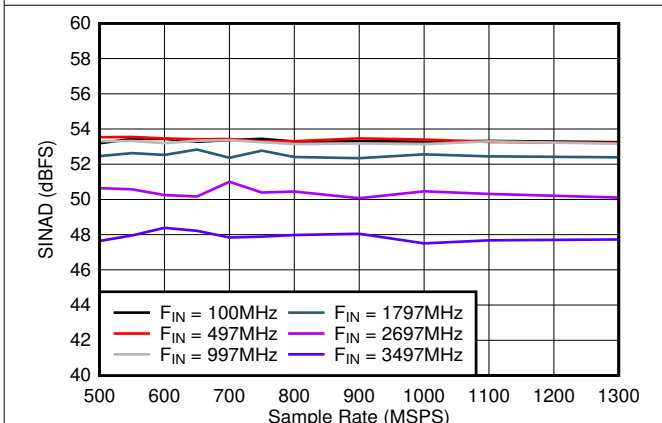
Figure 7-23. SINAD vs Sample Rate
