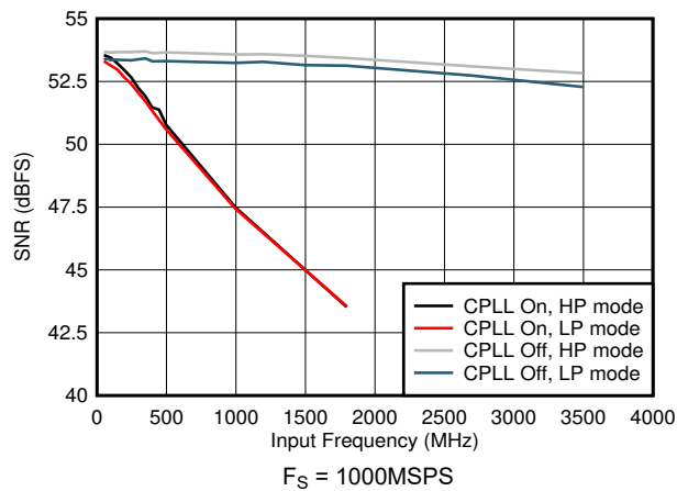
Figure 7-66. SNR vs Input Frequency and CPLL
