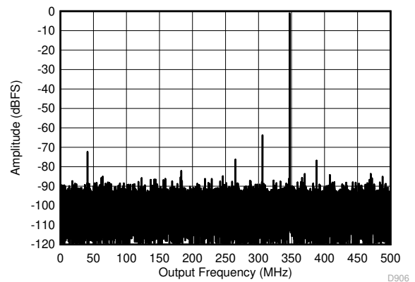
F_S = 1000\text{MSPS} , Low Power Mode Figure 7-12. Single Tone FFT at 347 MHz and -1 dBFS
