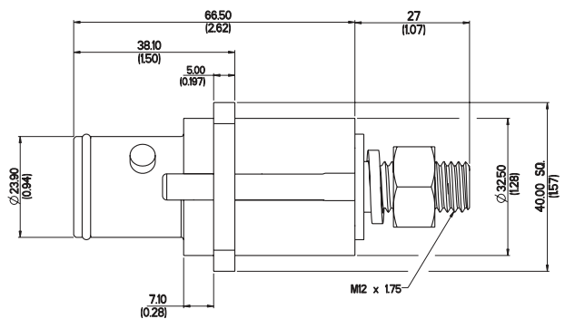
Male Panel Pin Order code- SNFM-P-TP-XX
