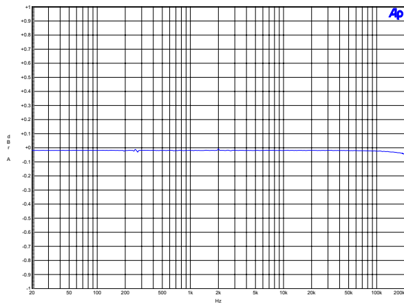
Figure 3. Frequency Response
