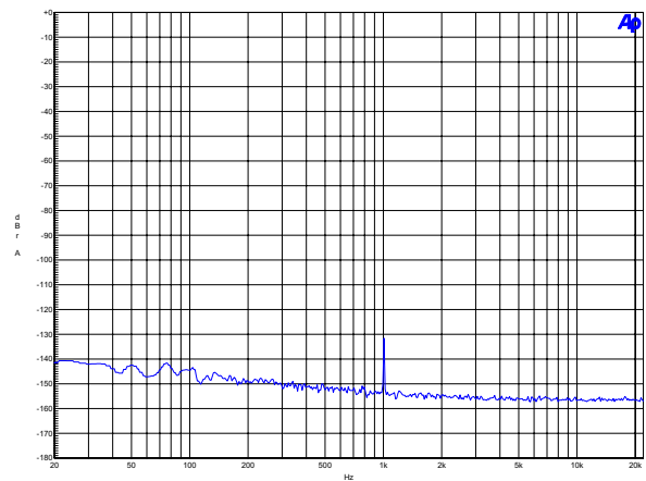
Figure 6. Crosstalk
