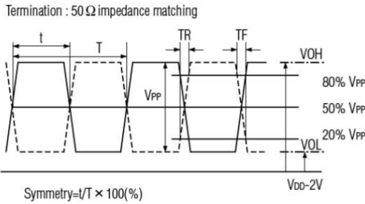
Figure 6) Output Waveform 1
