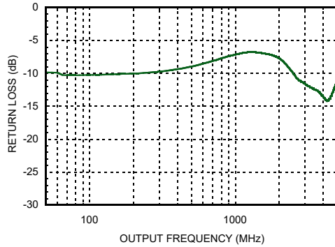
Figure 66. Auxiliary LO Differential Output Return Loss
