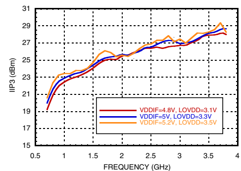
Figure 42. Low Side LO Input IP3 vs. VGATE=VDDIF
