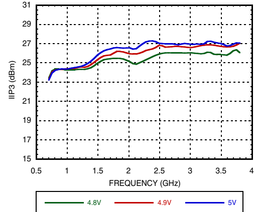
Input IP3 vs. VGATE [1]
