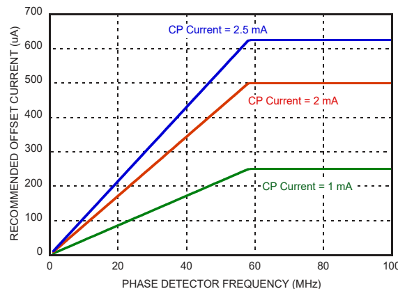
Recommended CP offset current vs PD frequency for typical CP gain currents. Calculated using EQ 9
