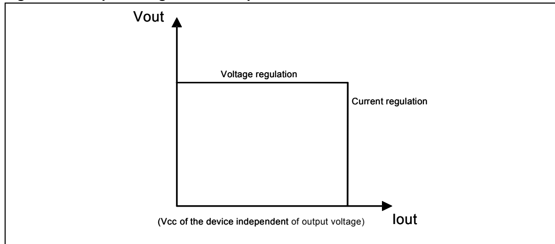
Figure 16. Output voltage versus output current
