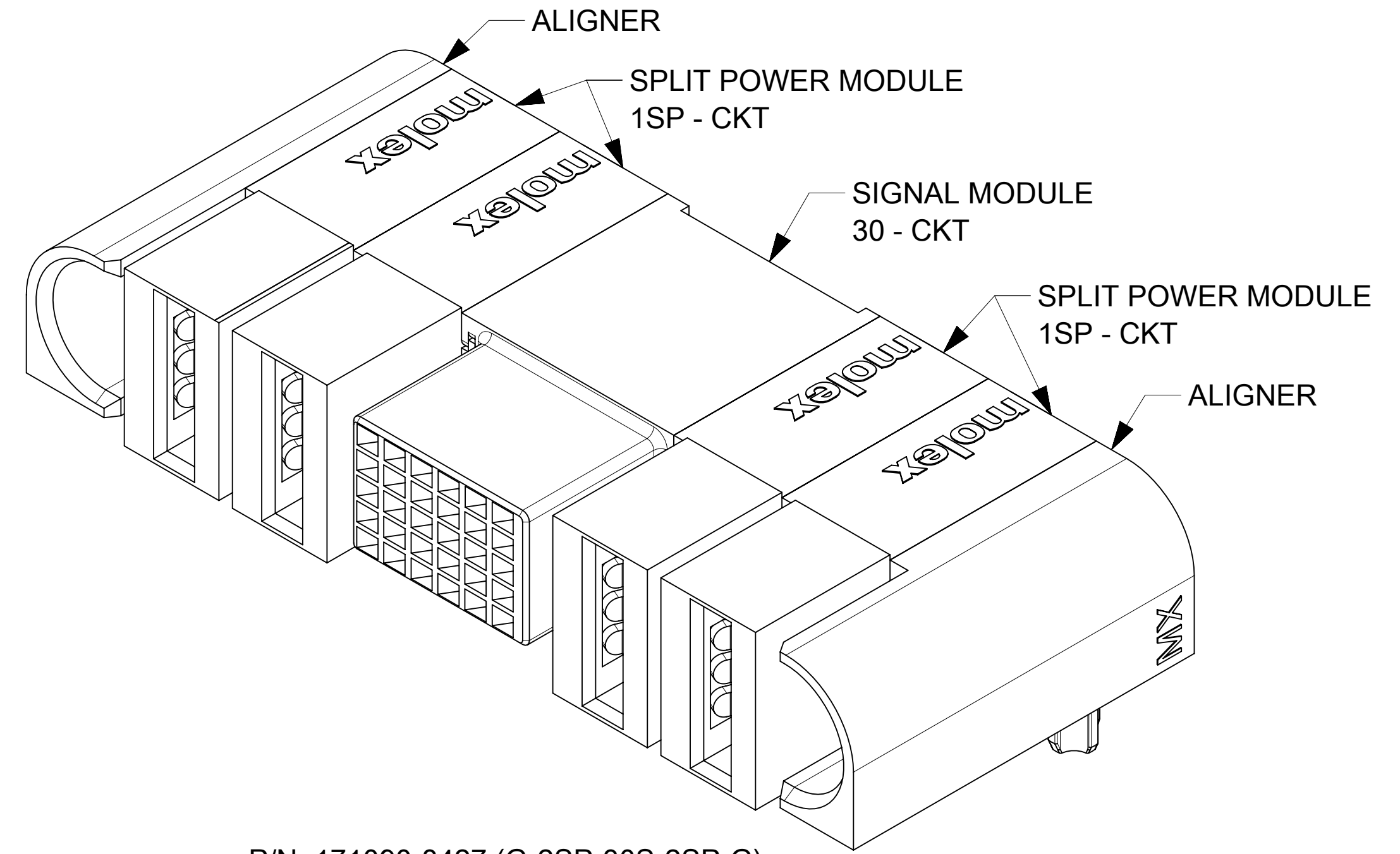
P/N: 171090-8427 (G-2SP-30S-2SP-G)
