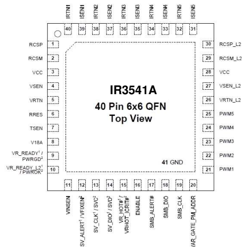
Figure 1: IR3541A Package Top View
