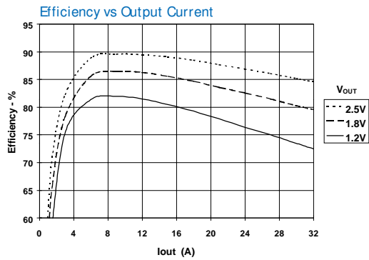
Performance Characteristics, V_{IN}=5.0V (See Note A)
