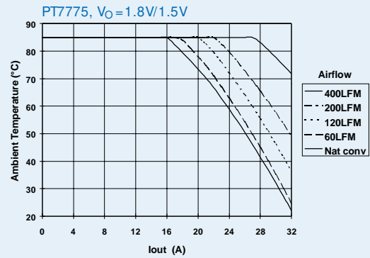
Safe Operating Area, V_{IN}=5.0V (See Note B)
