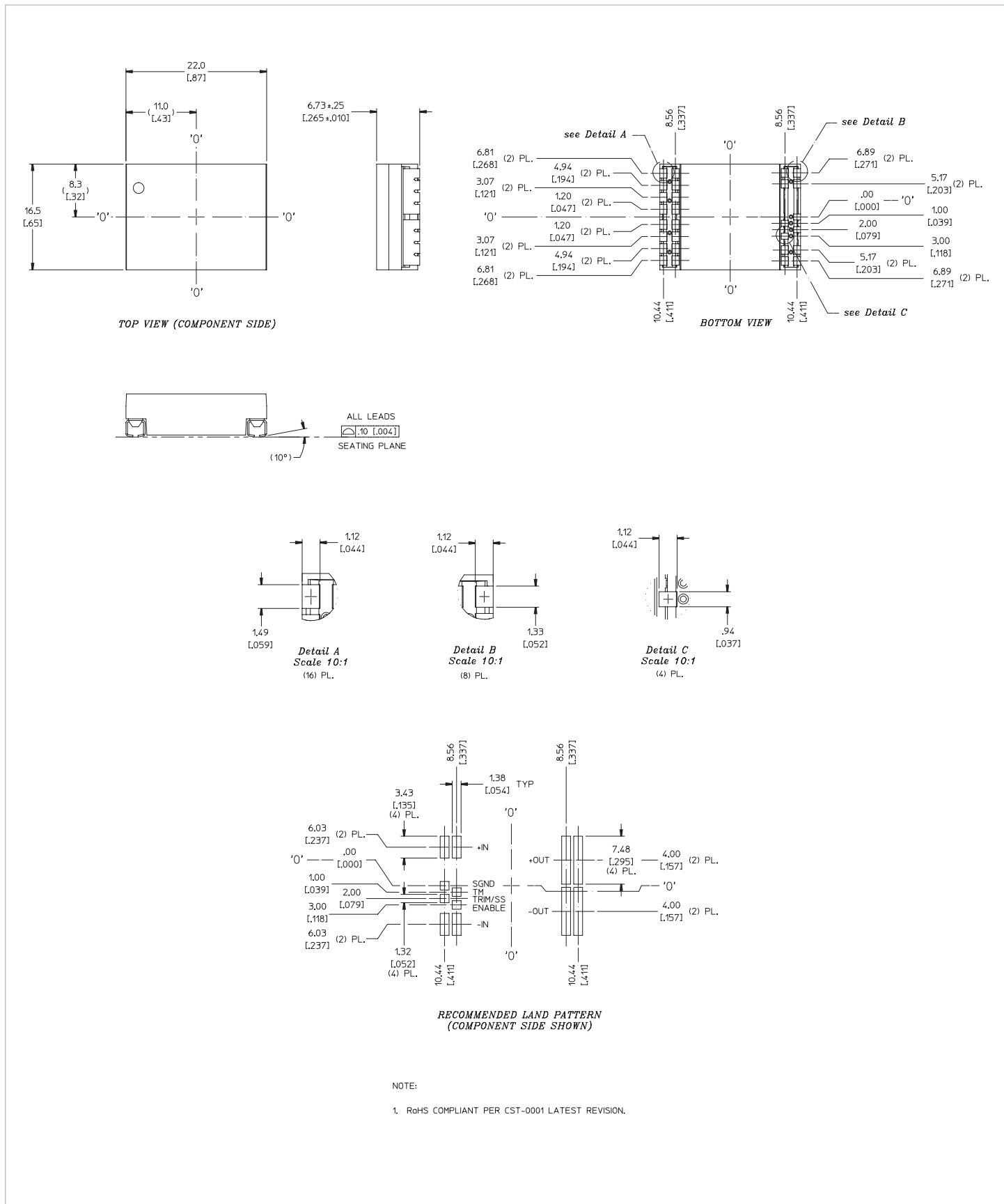
Figure 43 — Package outline & recommended PCB land pattern
