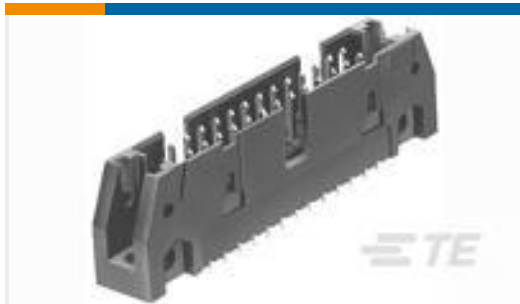
TE Part #5102155-6 A/L UNIV HDR 26P VERT
