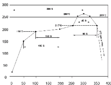
Figure 1 Resistance to soldering reflow heat test condition
