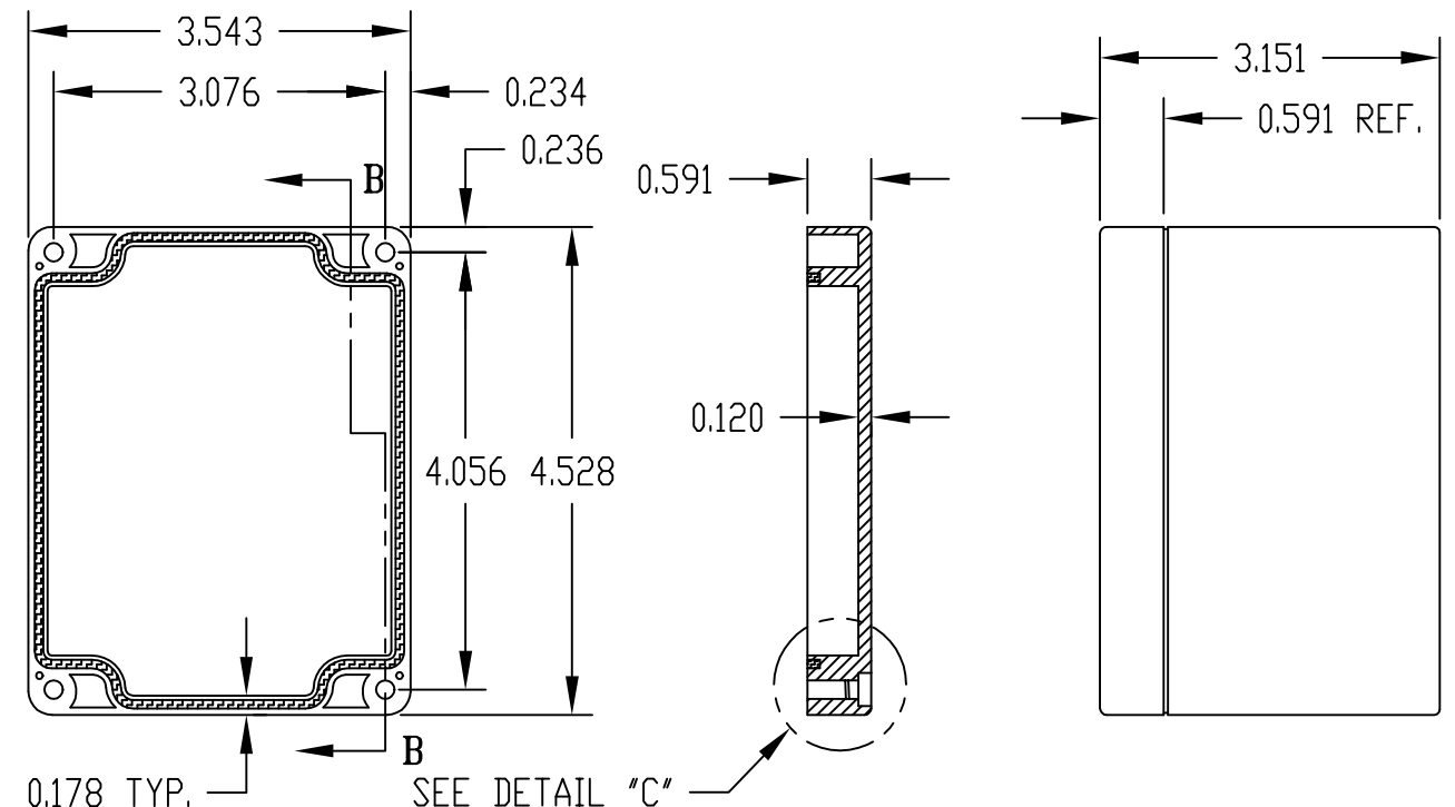
SECTION "B-B"
