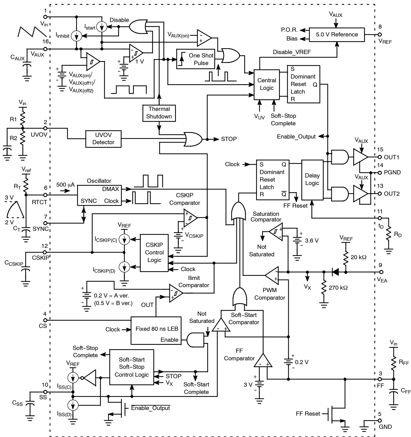
Figure 1. Detailed Block Diagram
