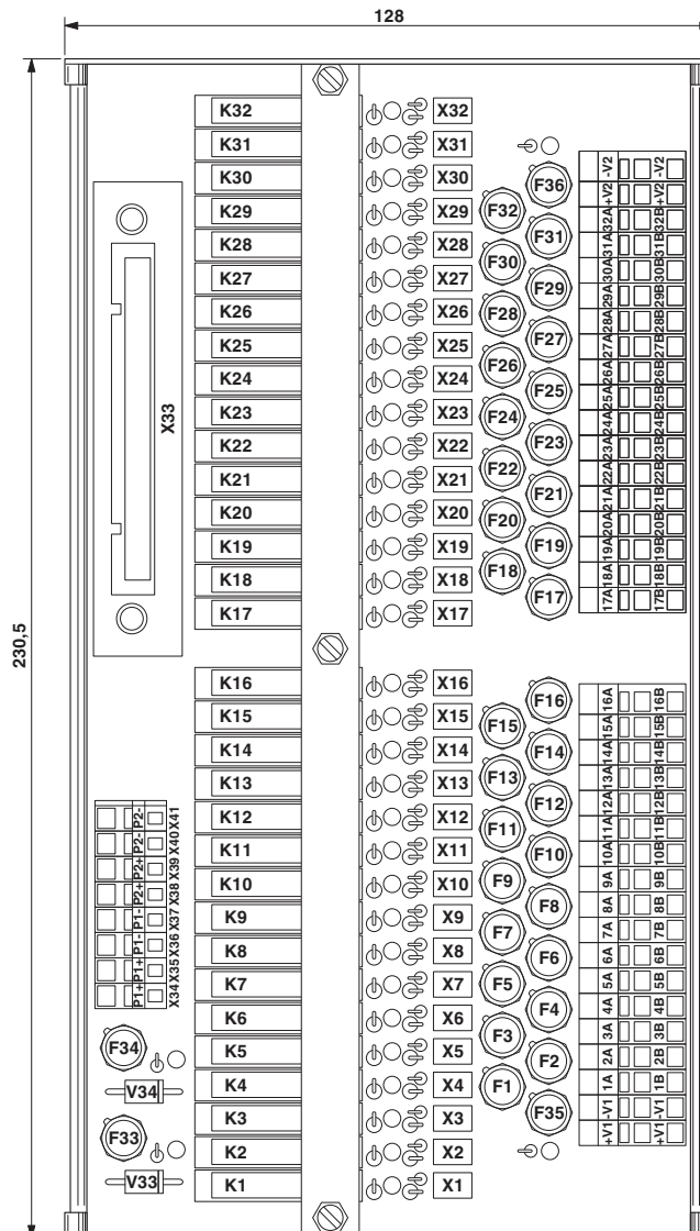
Dimensional drawing
