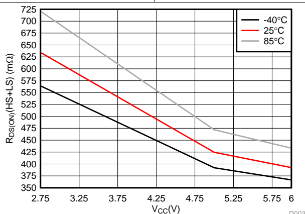
Figure 7. R_{DS(on)} HS + LS vs V_{VCC}
