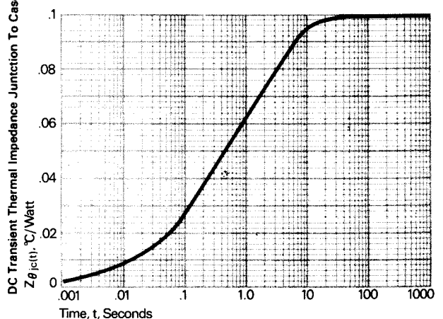
DC Transient Thermal Impedance VS. Time
