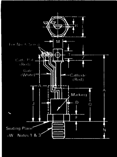
T70 Outline
