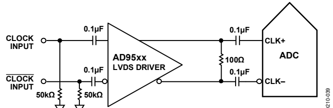
Figure 57. Differential LVDS Sample Clock (Up to 640 MHz)
