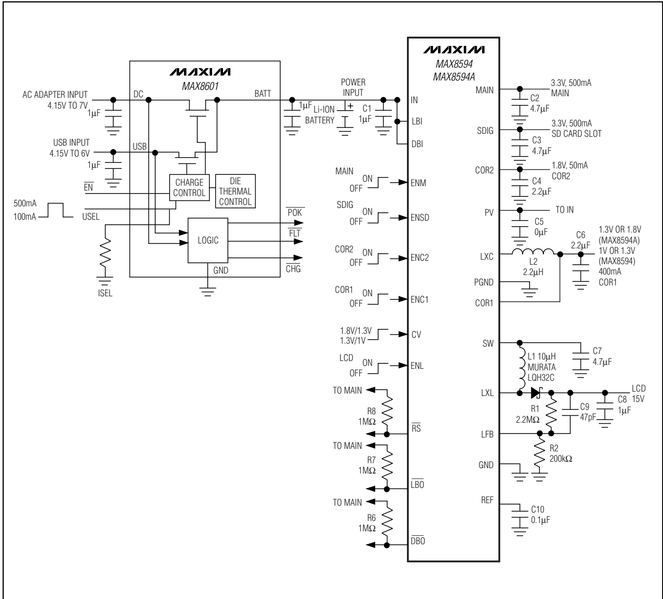
Figure 1. Typical Application Circuit with Charger
