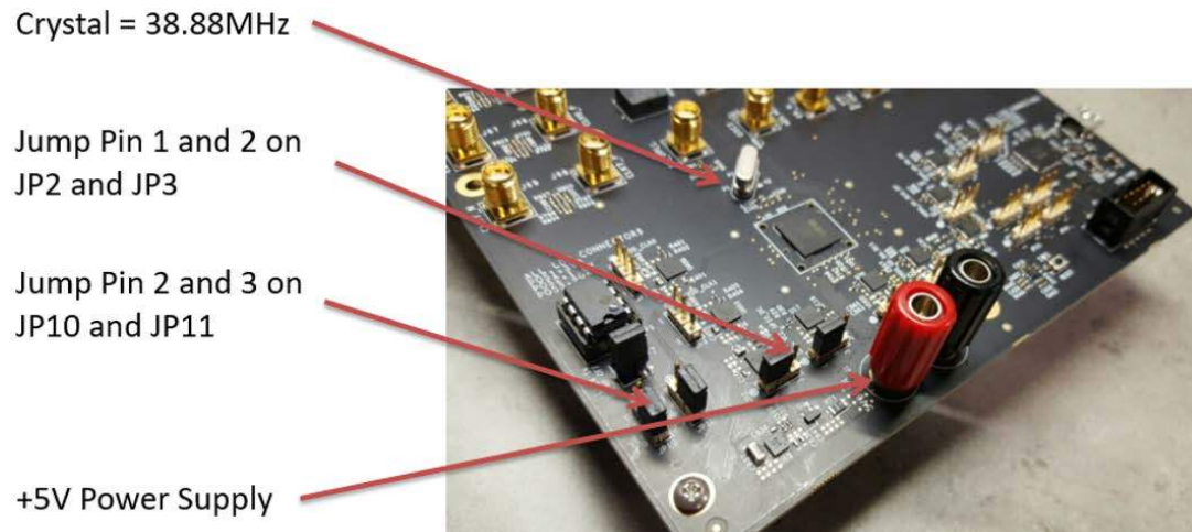
Figure 4. Board Setting for Default Operation
