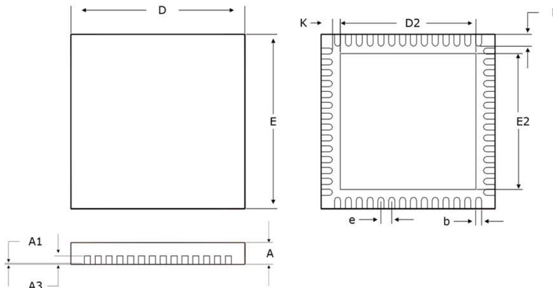
Figure 5-1. PD69208T4 Package Drawing (56 Pin QFN 8 mm × 8 mm)
