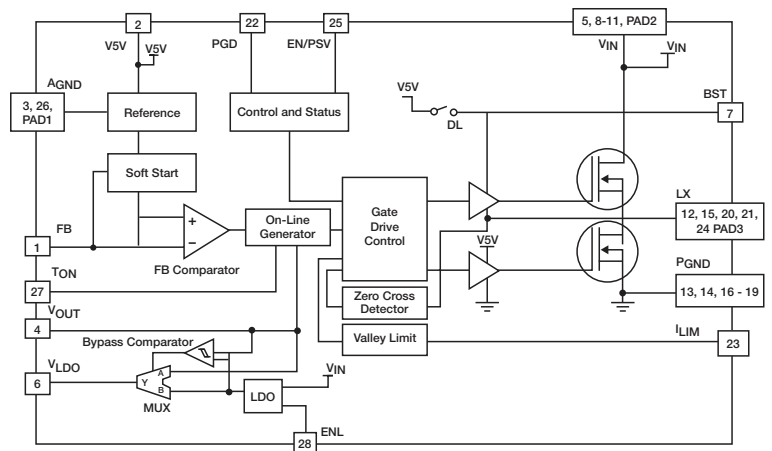
SiC414CD block diagram
