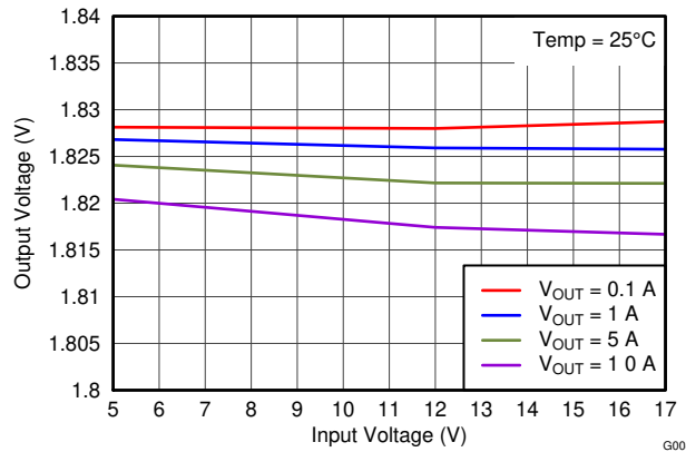
Figure 2-3. TPS54020EVM-082 Line Regulation
