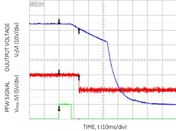
Figure 12. PFV alarmed 19.6ms prior to Vo < 40V, output load: 38A, V IN = 185V AC .
