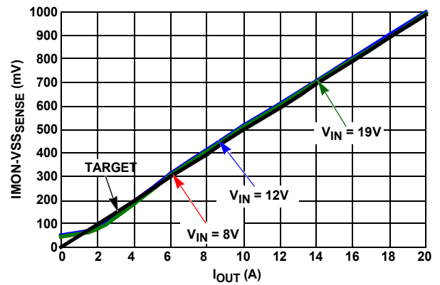
FIGURE 39. IMON, V_{ID} = 1.2375
