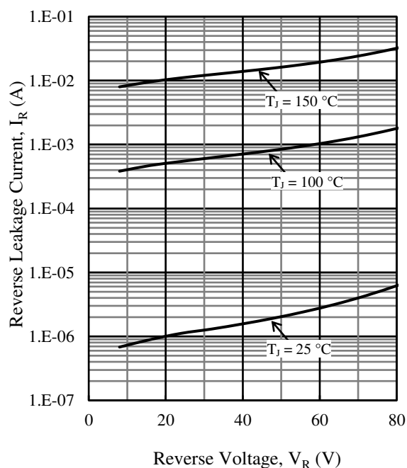
Figure 6. Typical Characteristics: I_R vs. V_R
