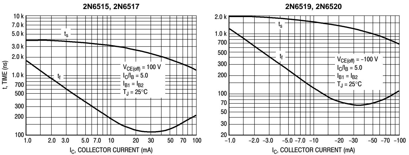
Figure 8. Turn-Off Time
