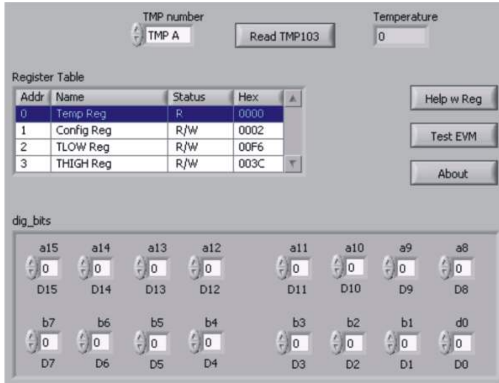
Figure 20. TMP103EVM Software: Register Tab
