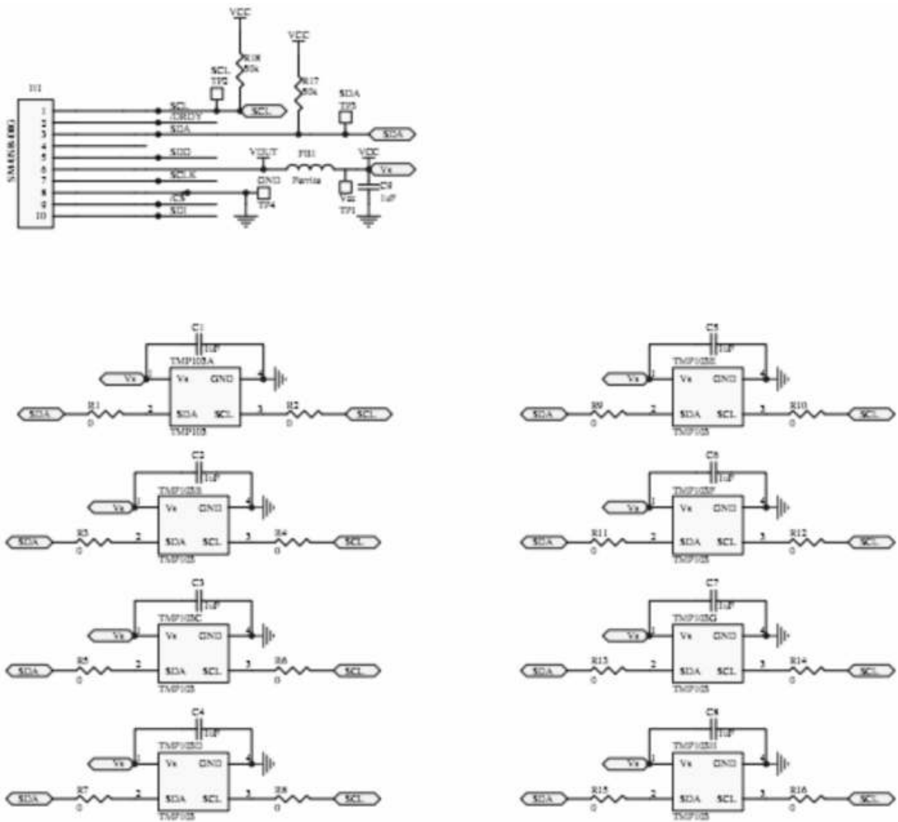
Figure 22. TMP103EVM Schematic
